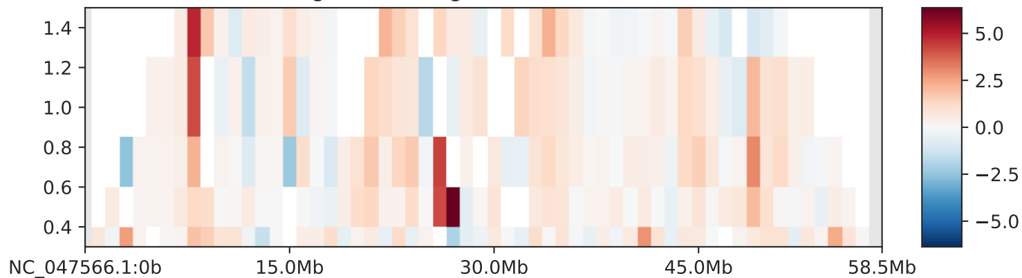
signif (HiCcompare)
