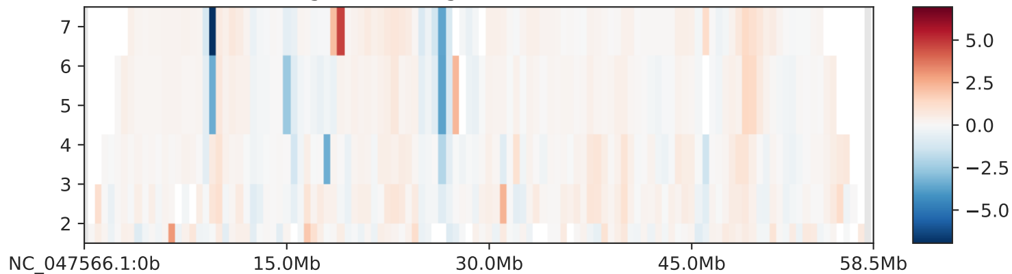
signif (HiCcompare)
