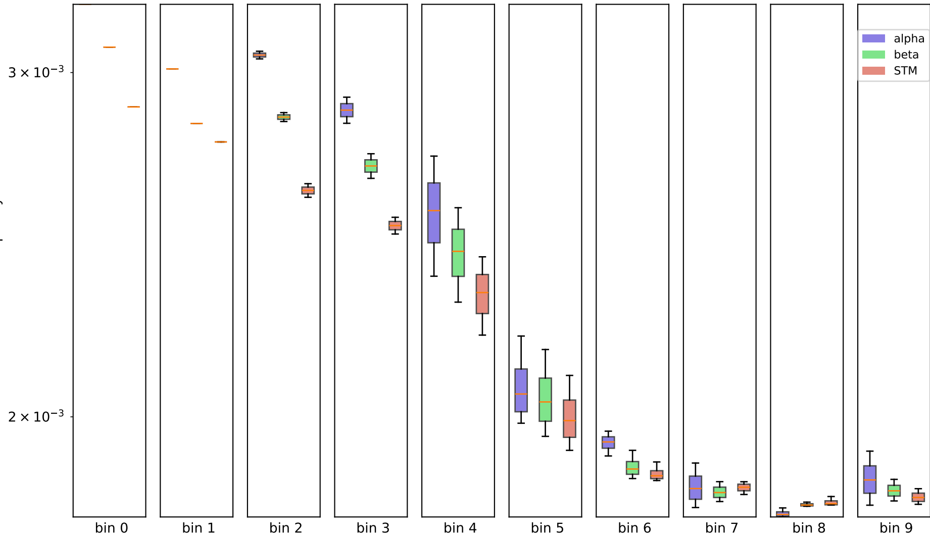
1Mb - chr1, (10 bins)
