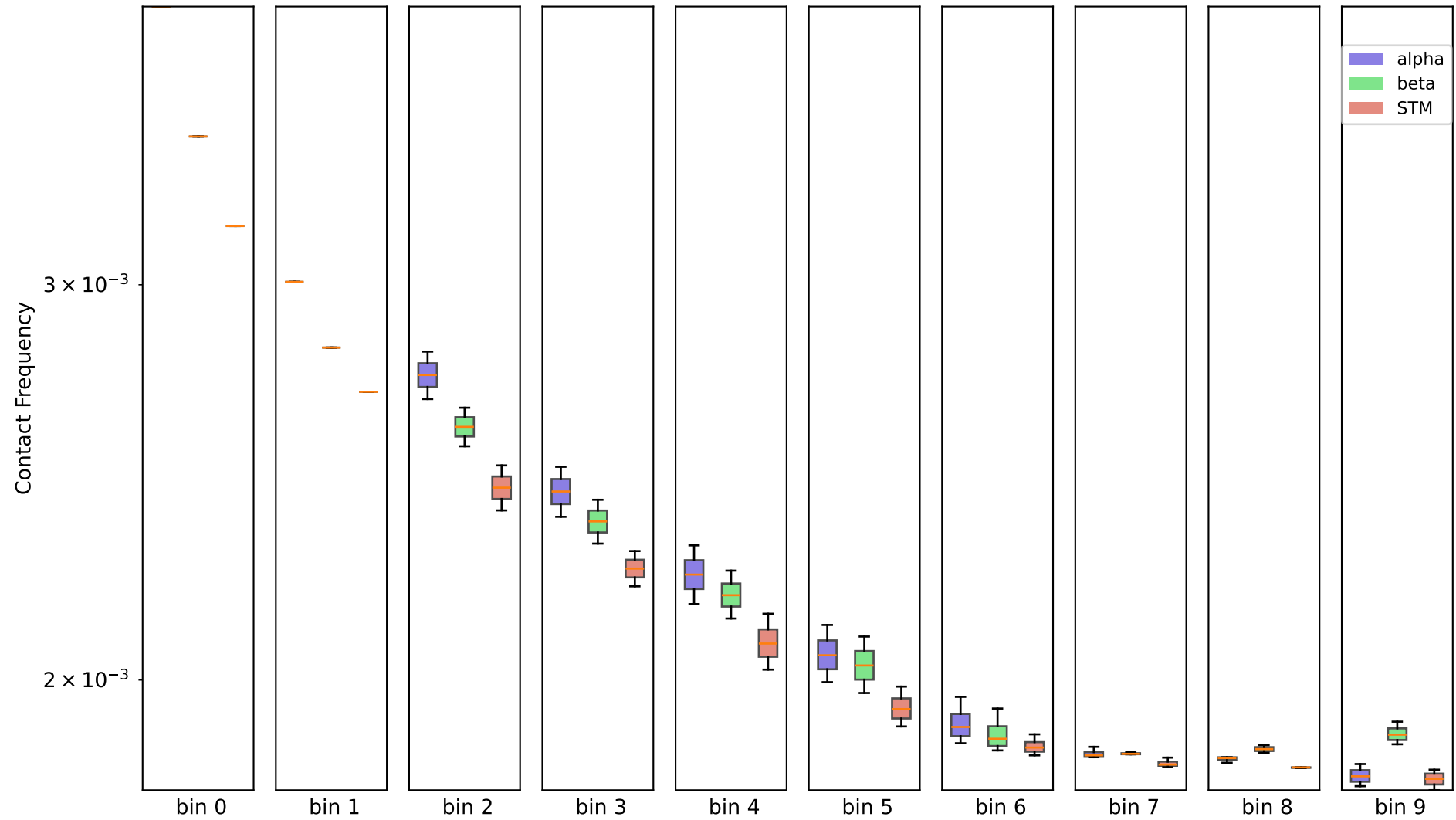
1Mb - chr7, (10 bins)
