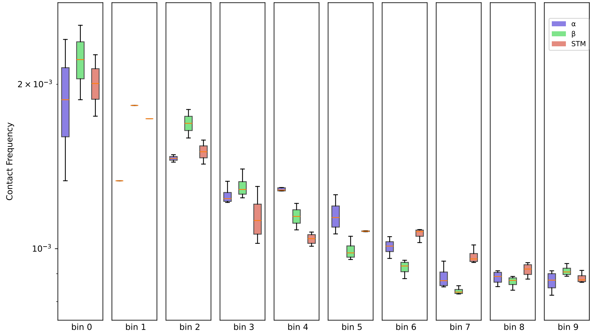
500kb - chr6, (10 bins) - 250k contacts per sample
