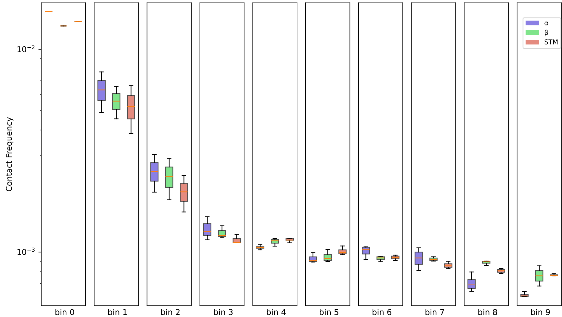
500kb - chr4, (10 bins) - 250k contacts per sample
