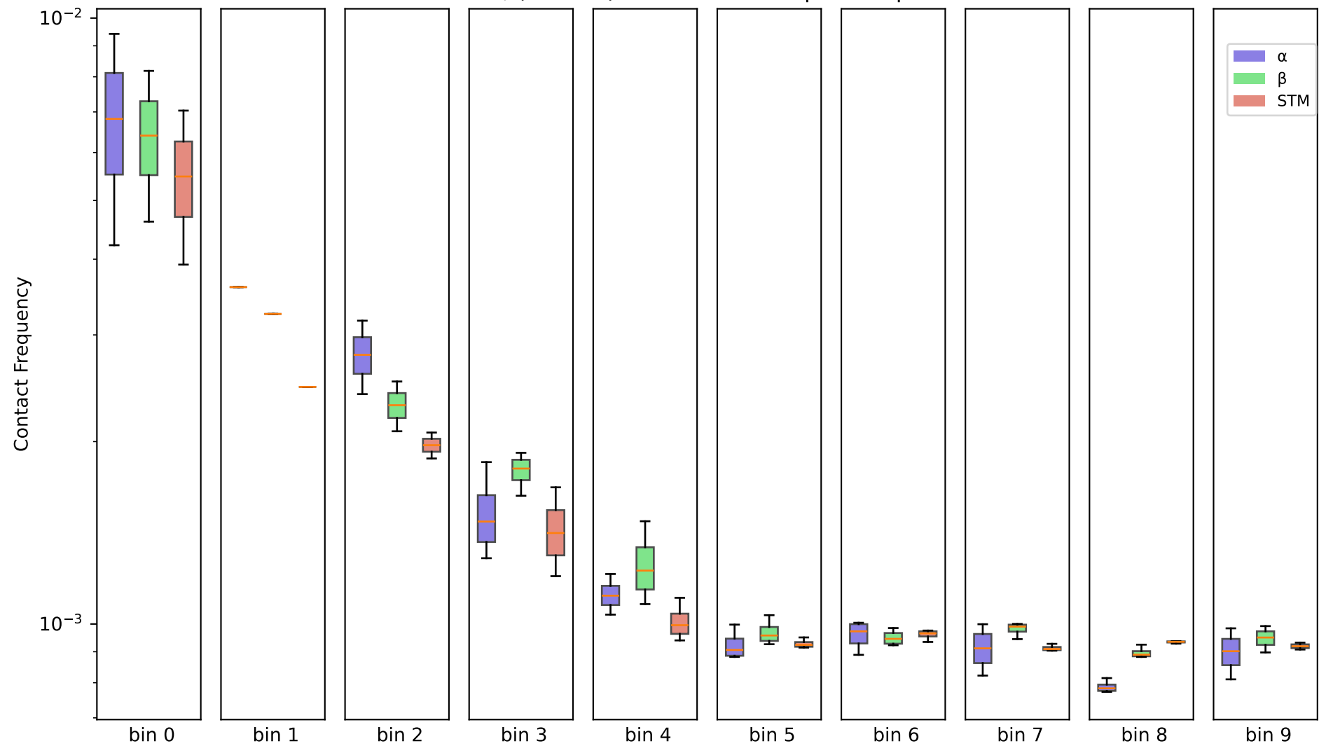
500kb - chr8, (10 bins) - 250k contacts per sample
