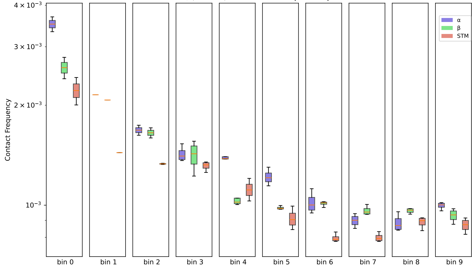
500kb - chr3, (10 bins) - 250k contacts per sample
