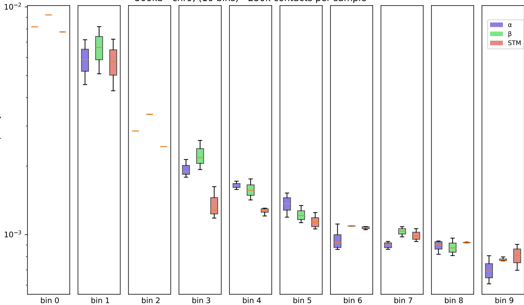
500kb - chr9, (10 bins) - 250k contacts per sample
