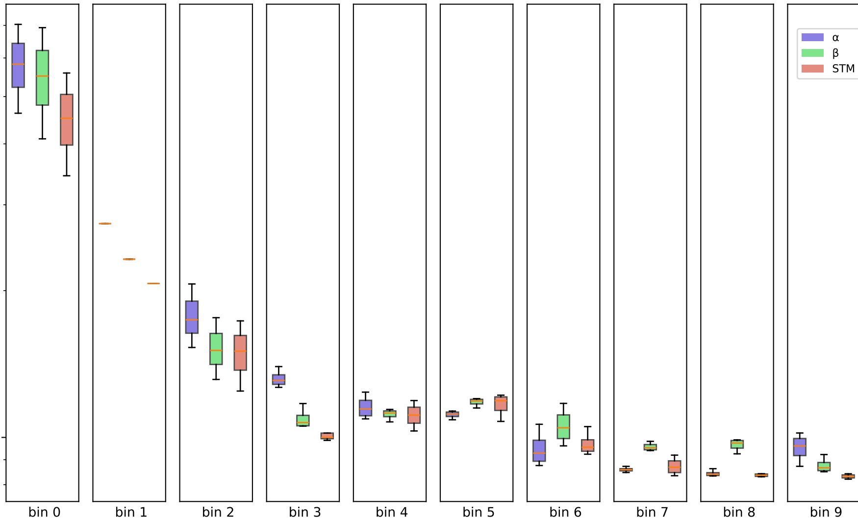
500kb - chr5, (10 bins) - 250k contacts per sample
