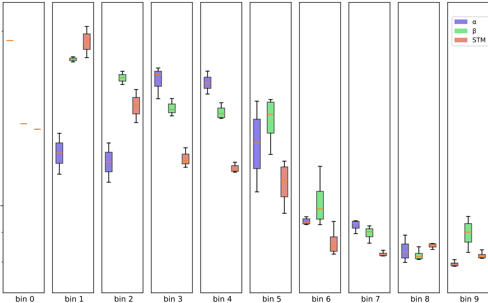
500kb - chr1, (10 bins) - 250k contacts per sample
