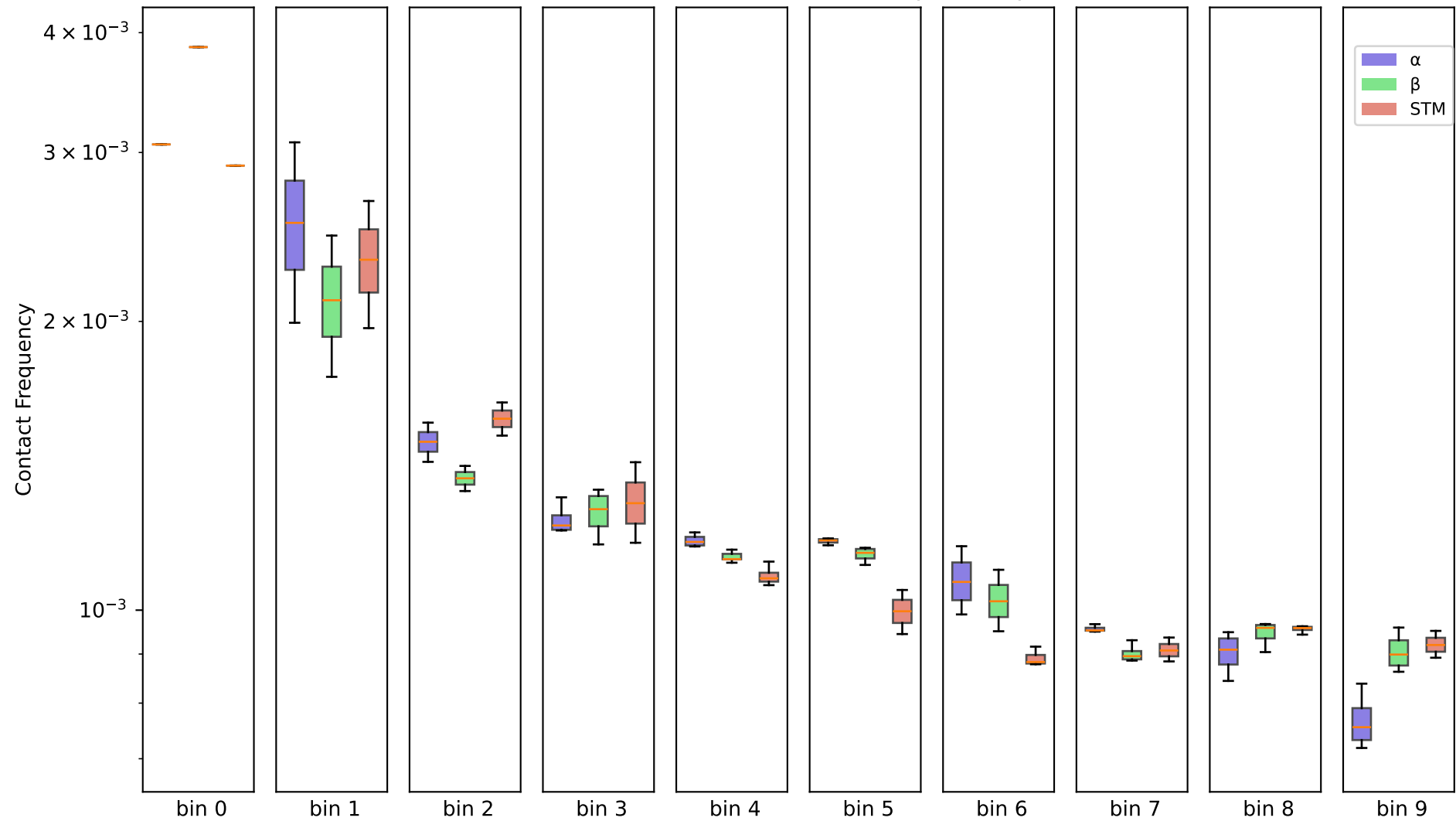
500kb - chr10, (10 bins) - 250k contacts per sample
