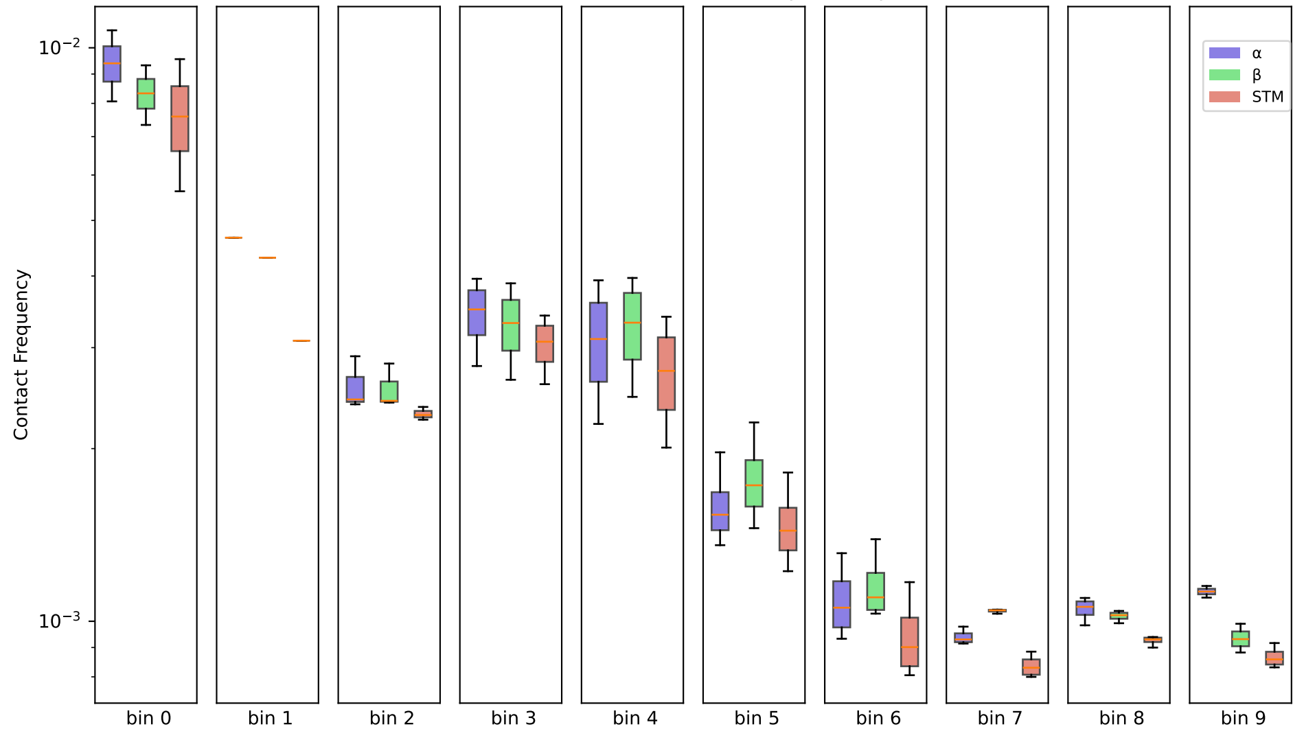
500kb - chr2, (10 bins) - 250k contacts per sample
