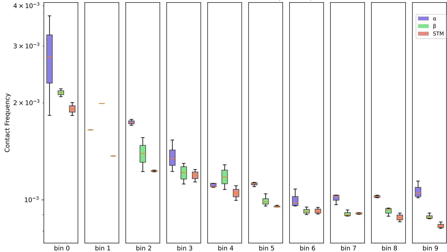
500kb - chr7, (10 bins) - 250k contacts per sample
