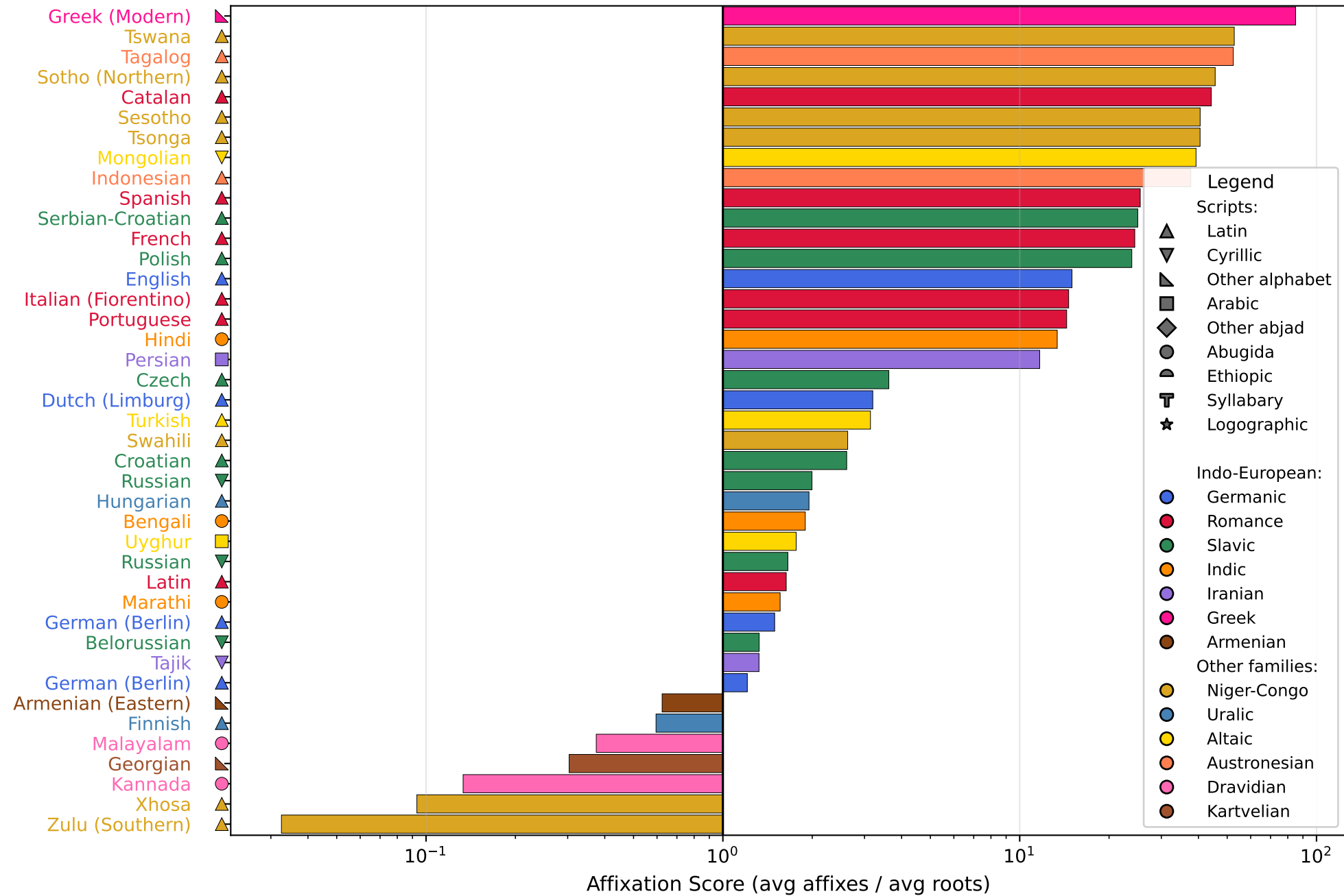
Affixation Score (centered at 1)
