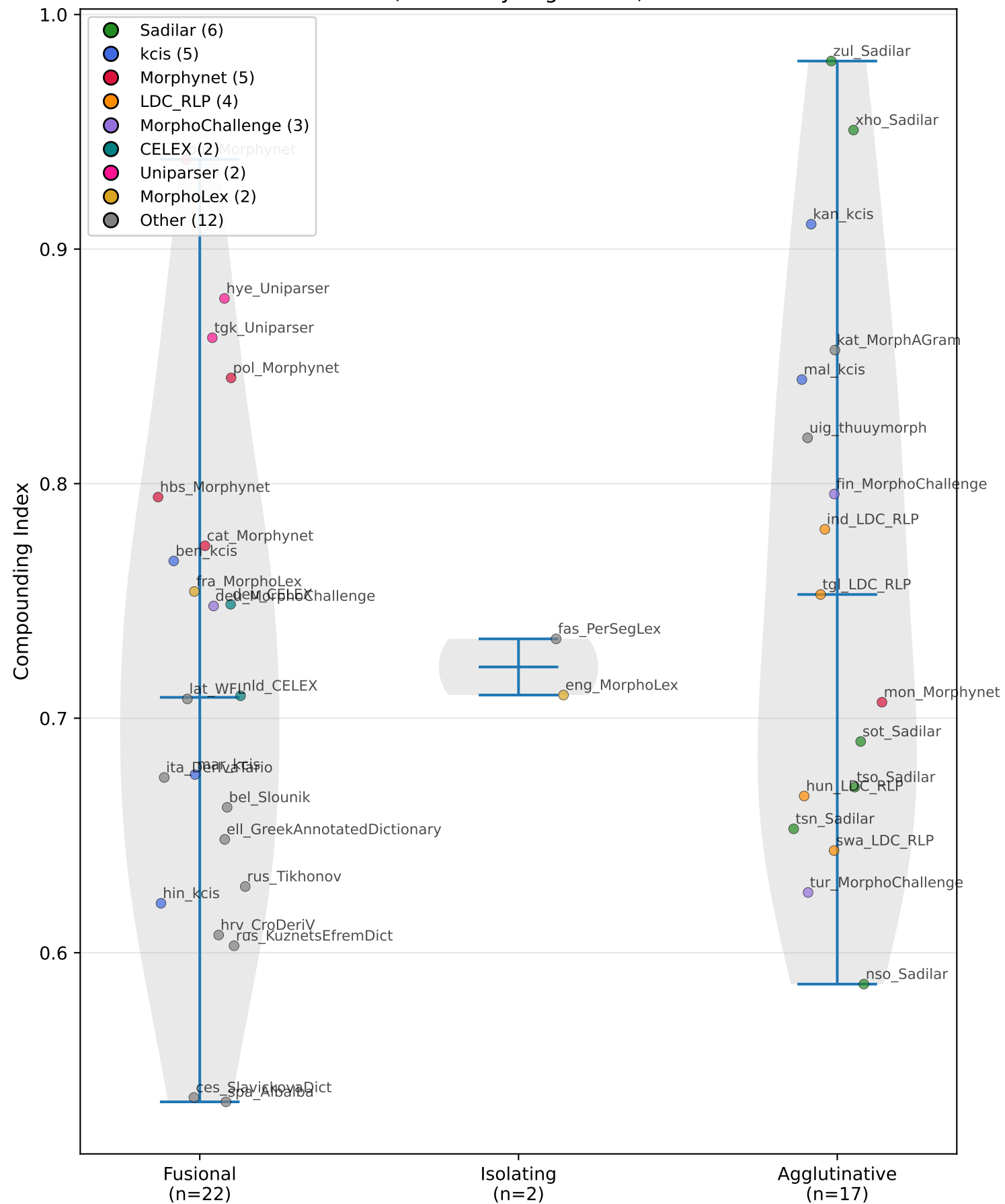
Compounding Index distribution by morphological typology (colored by segmentor)
