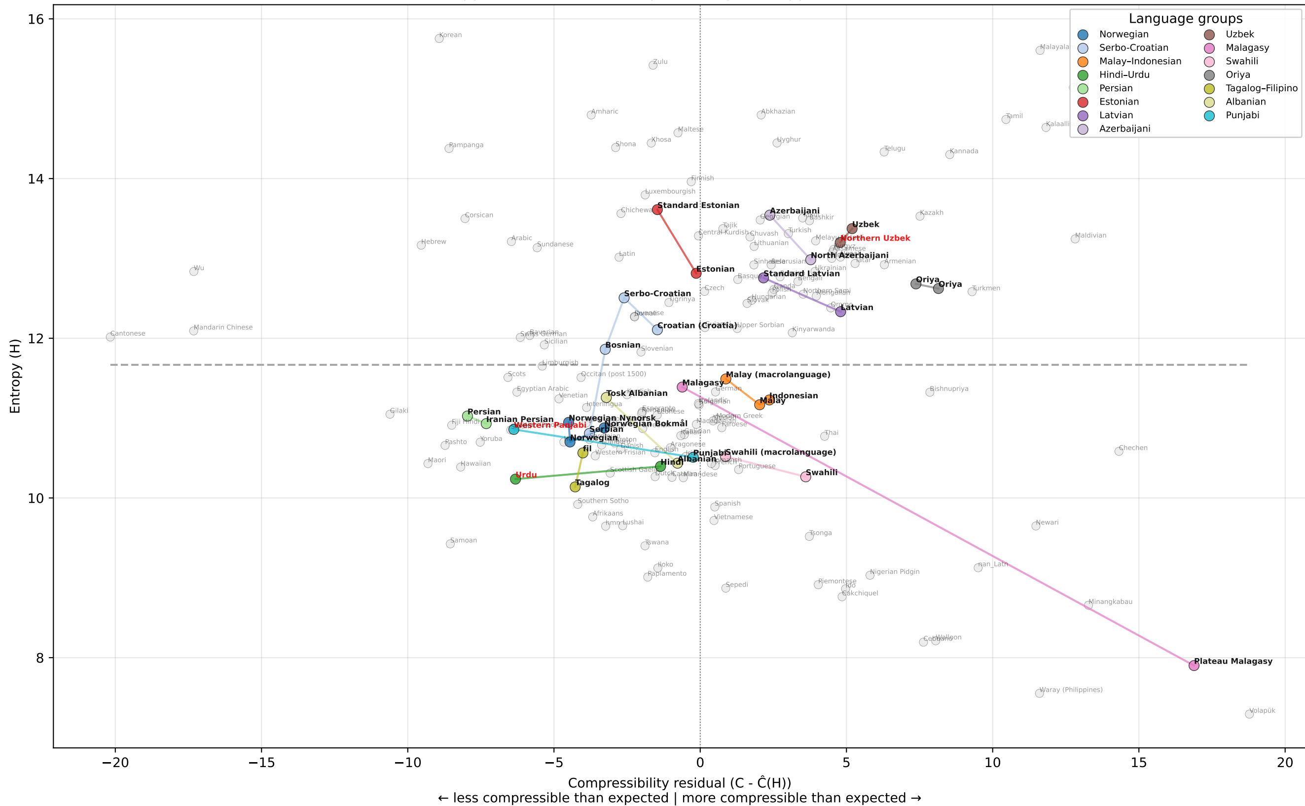
Entropy vs Residualized Compressibility (entropy effect removed)
