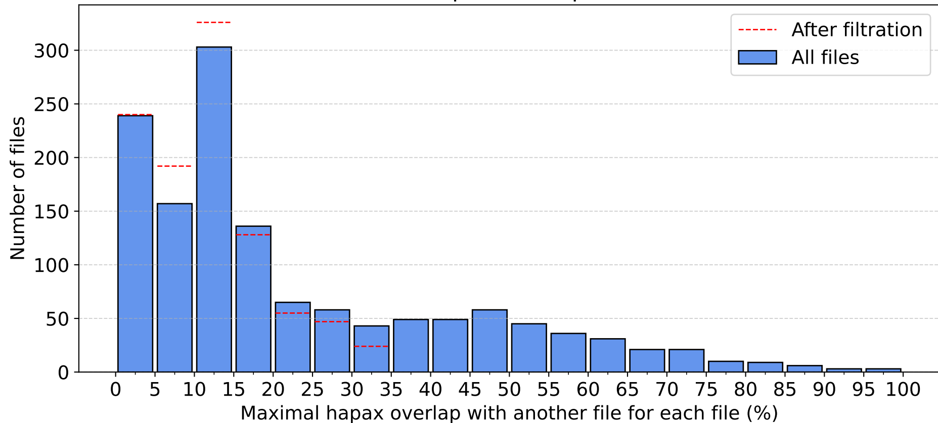
Distribution of maximal hapax overlap of a file with another file
