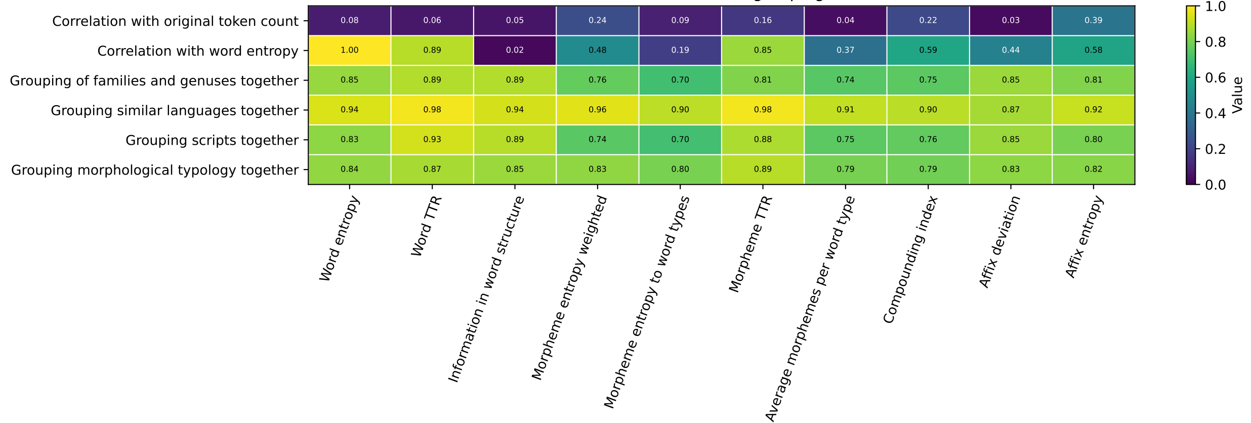
Metric correlations and grouping scores
