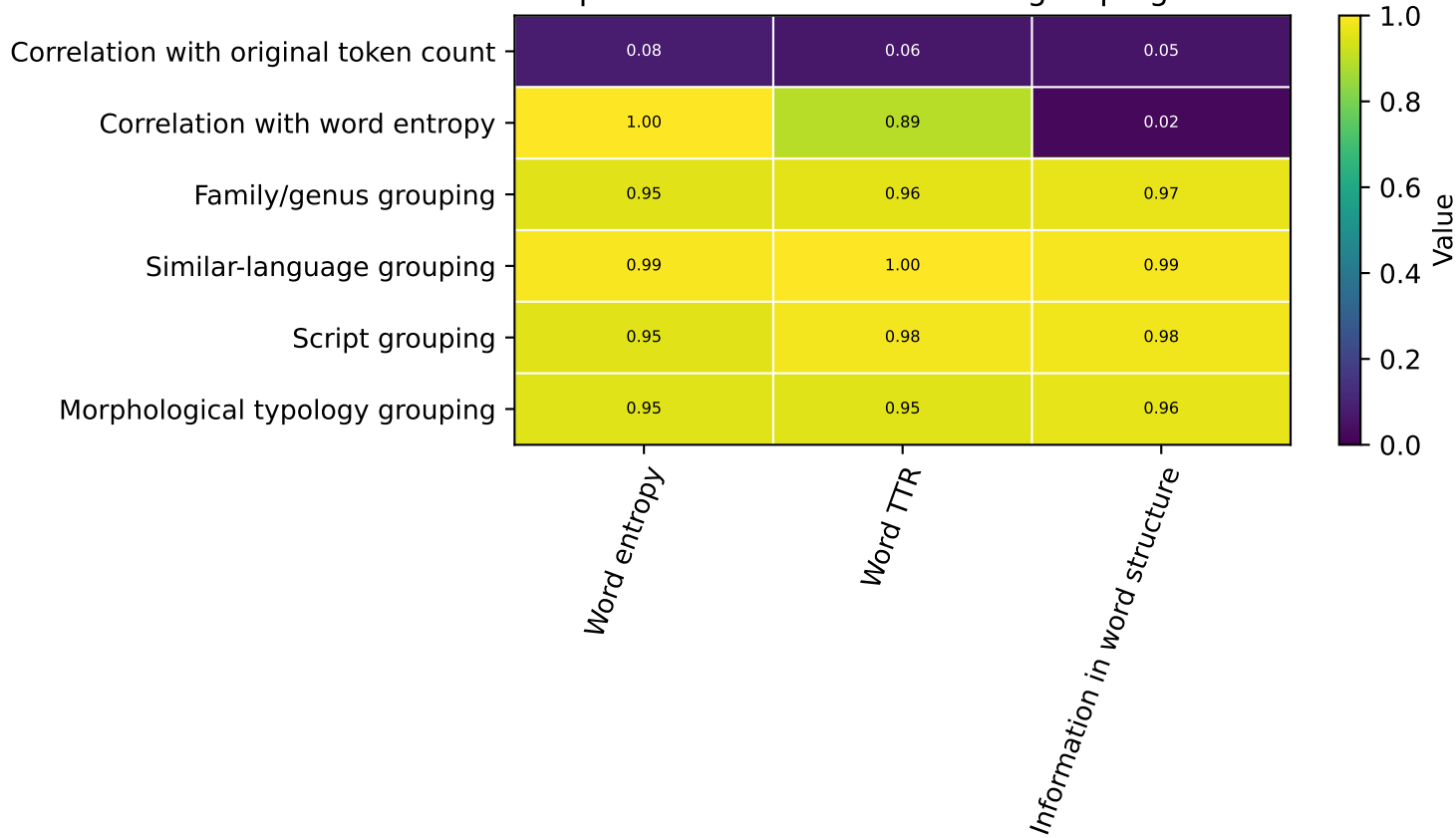
Corpus metric correlations and grouping scores
