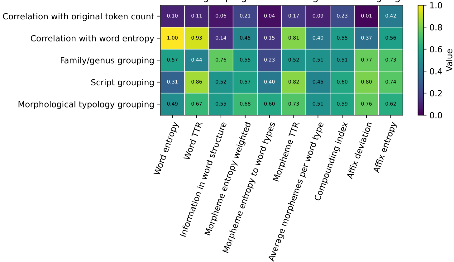
Stretched grouping scores on segmented languages
