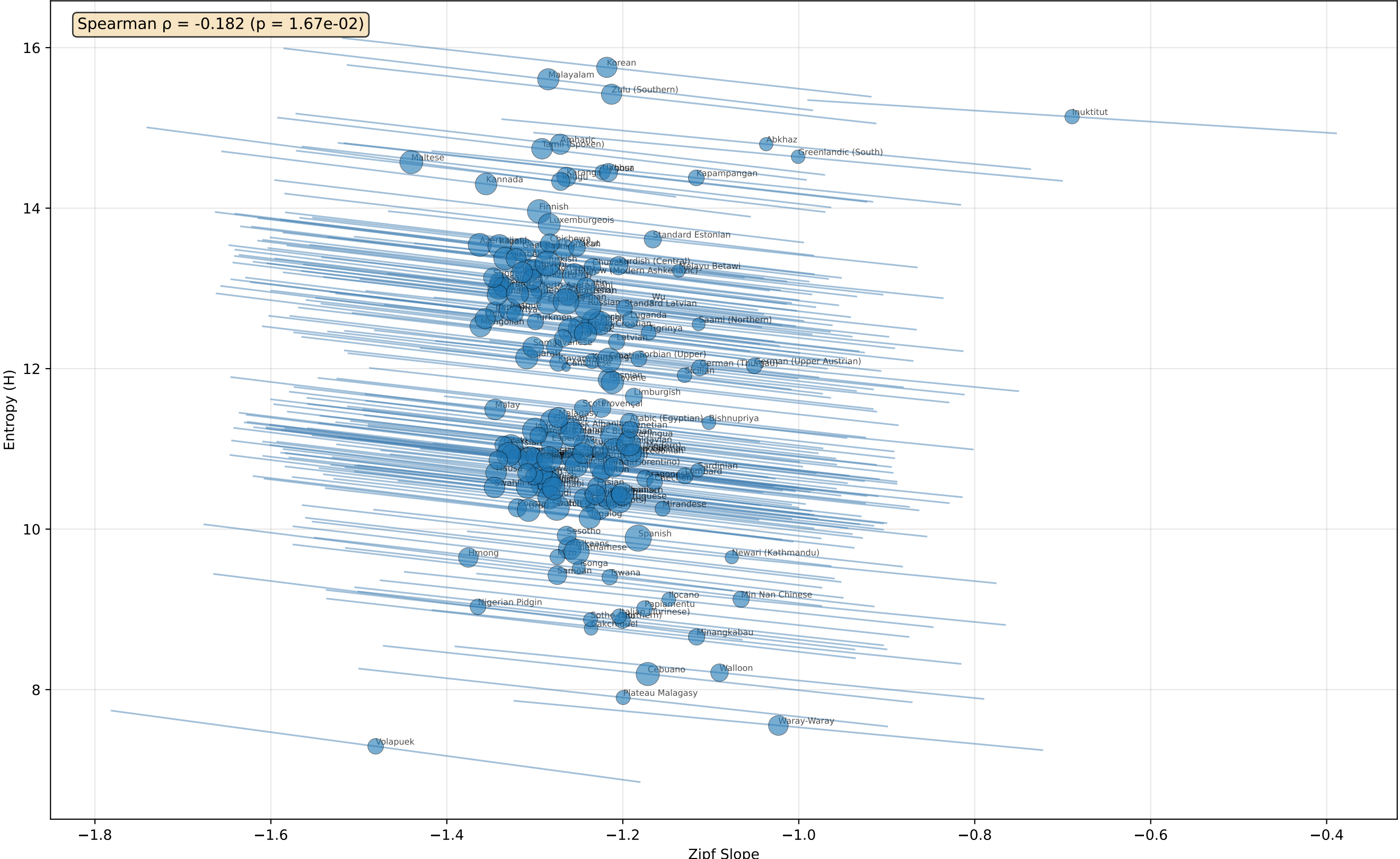
Zinf Slope vs Entropy — line segments show each language's
