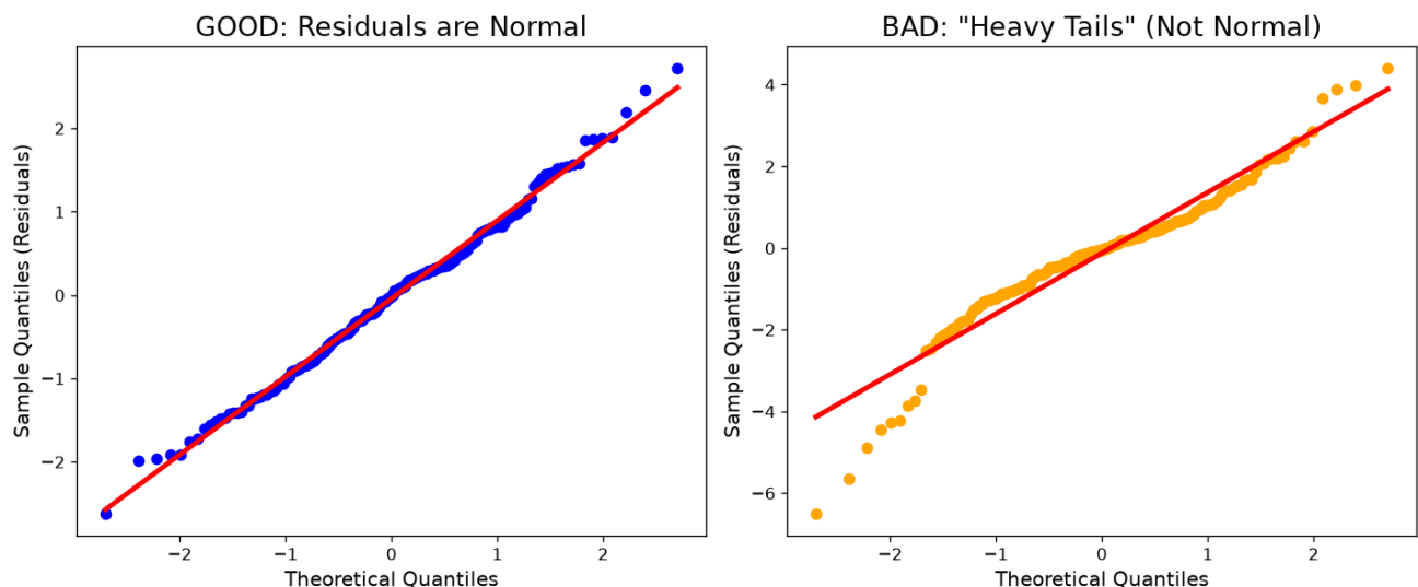
Q-Q Plot: Checking for Normal Residuals
