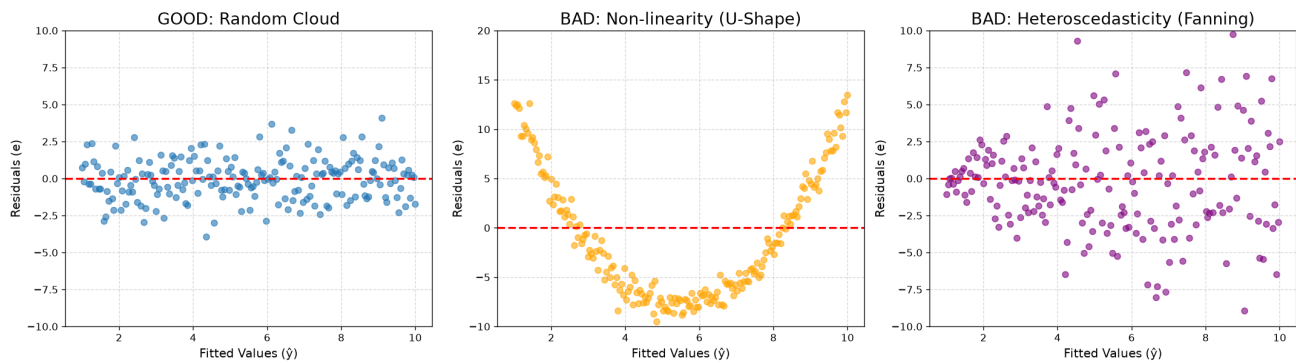
The Residuals vs. Fitted Plot: Good vs. Bad
