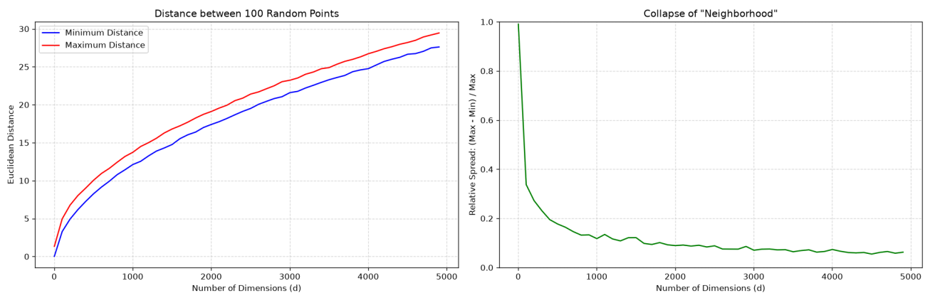
Illustration of the Curse of Dimensionality
