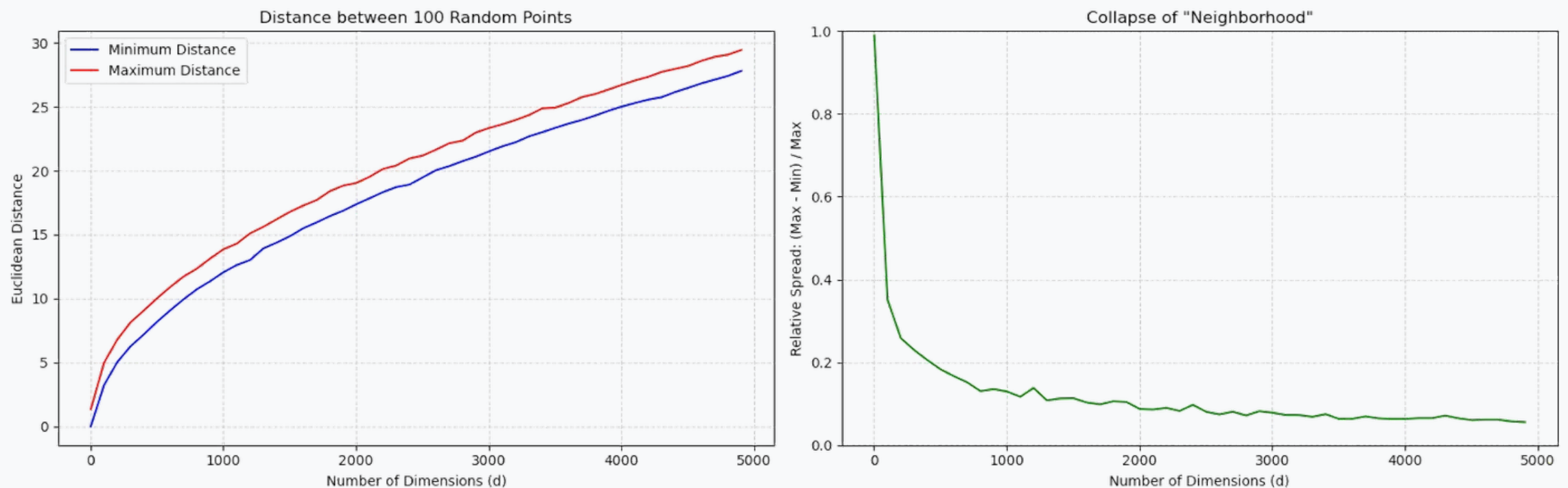
Illustration of the Curse of Dimensionality
