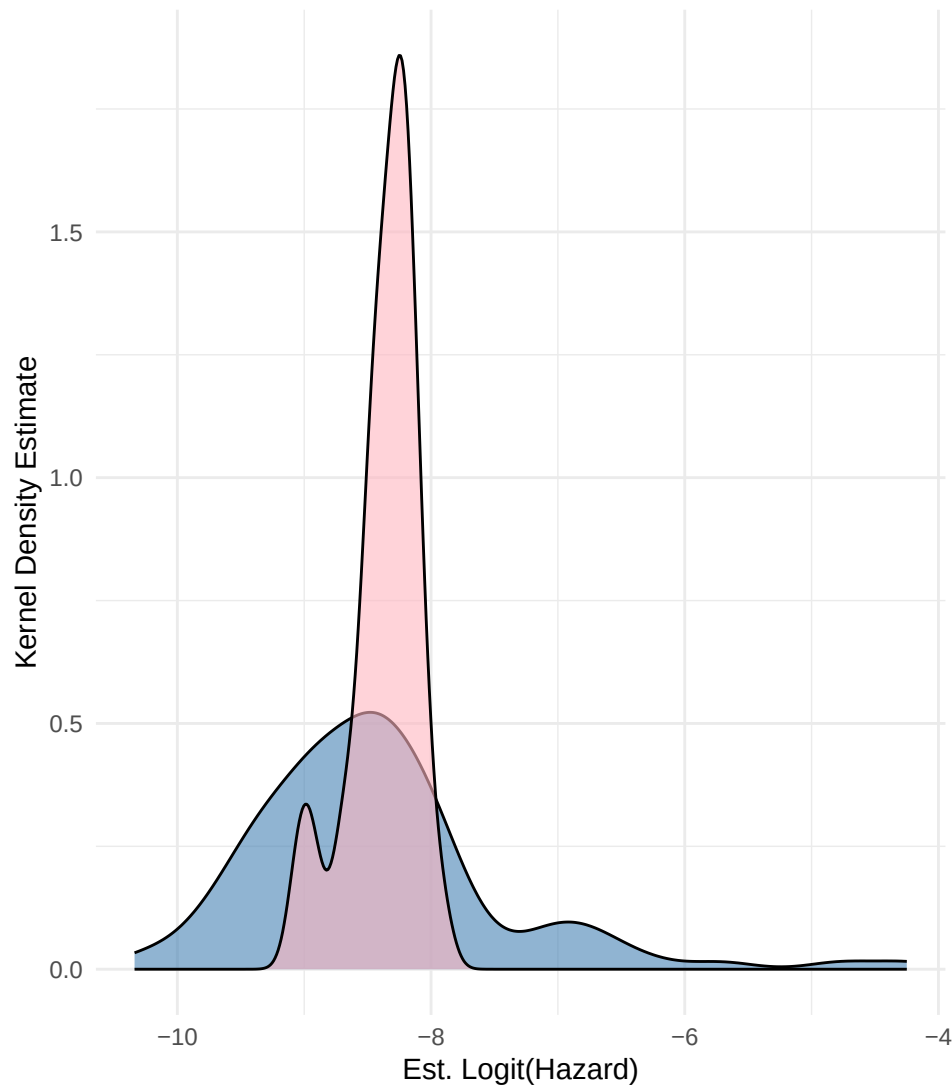
Overlapping Densities by last_invert
