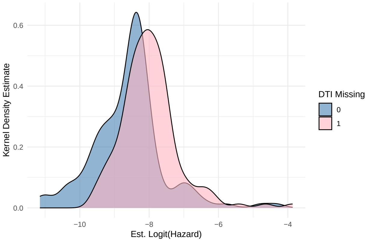
Densities of Logit Hazard for Missing vs. Non-Missing DTI
