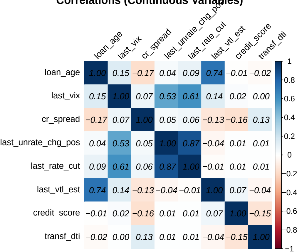
Correlations (Continuous variables)
