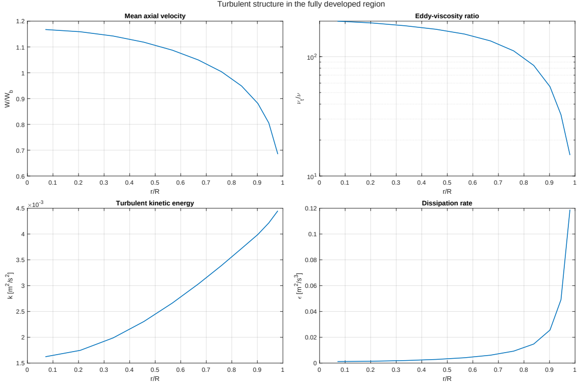
Figure 7: Radial structure of the standard k-\varepsilon solution in the developed region.
