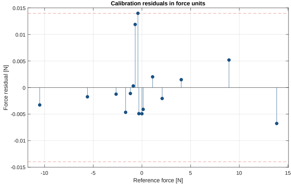
Figure 12: Calibration residuals after conversion to force units.
