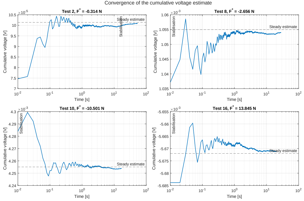
Figure 13: Convergence of the cumulative voltage estimate for four representative calibration tests.
