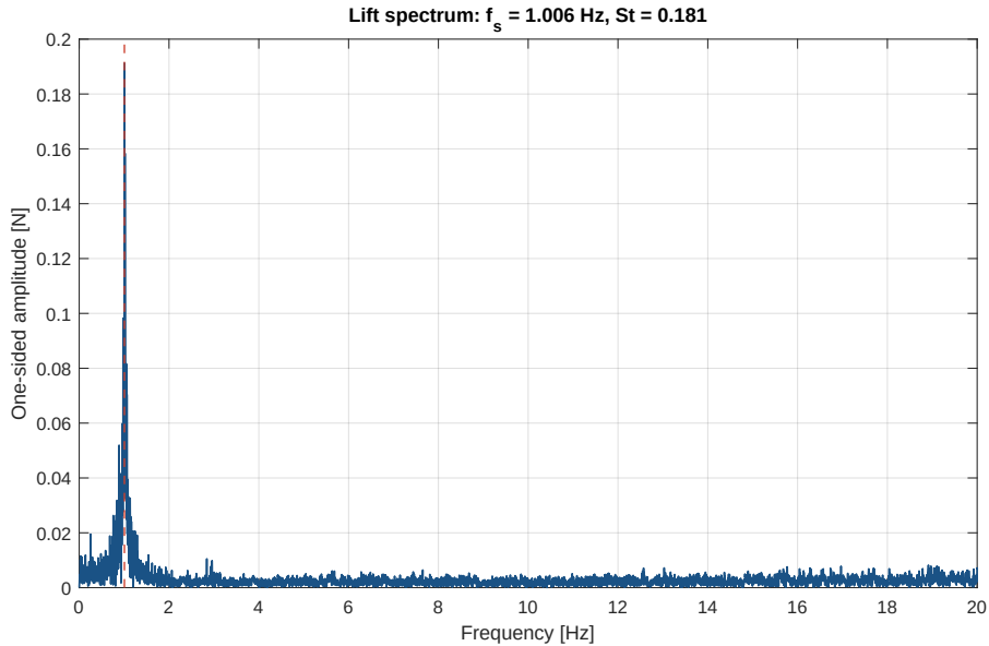
Figure 19: One-sided amplitude spectrum of the corrected lift signal.
