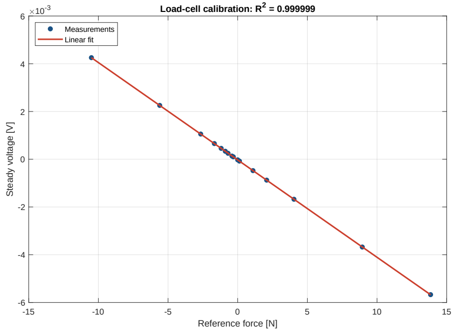
Figure 11: Static load-cell calibration from sixteen reference loads.
