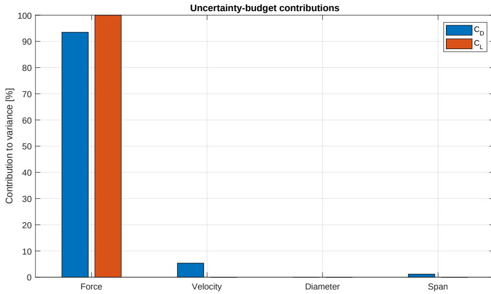
Figure 20: Contributions to the propagated variance of the force coefficients.
