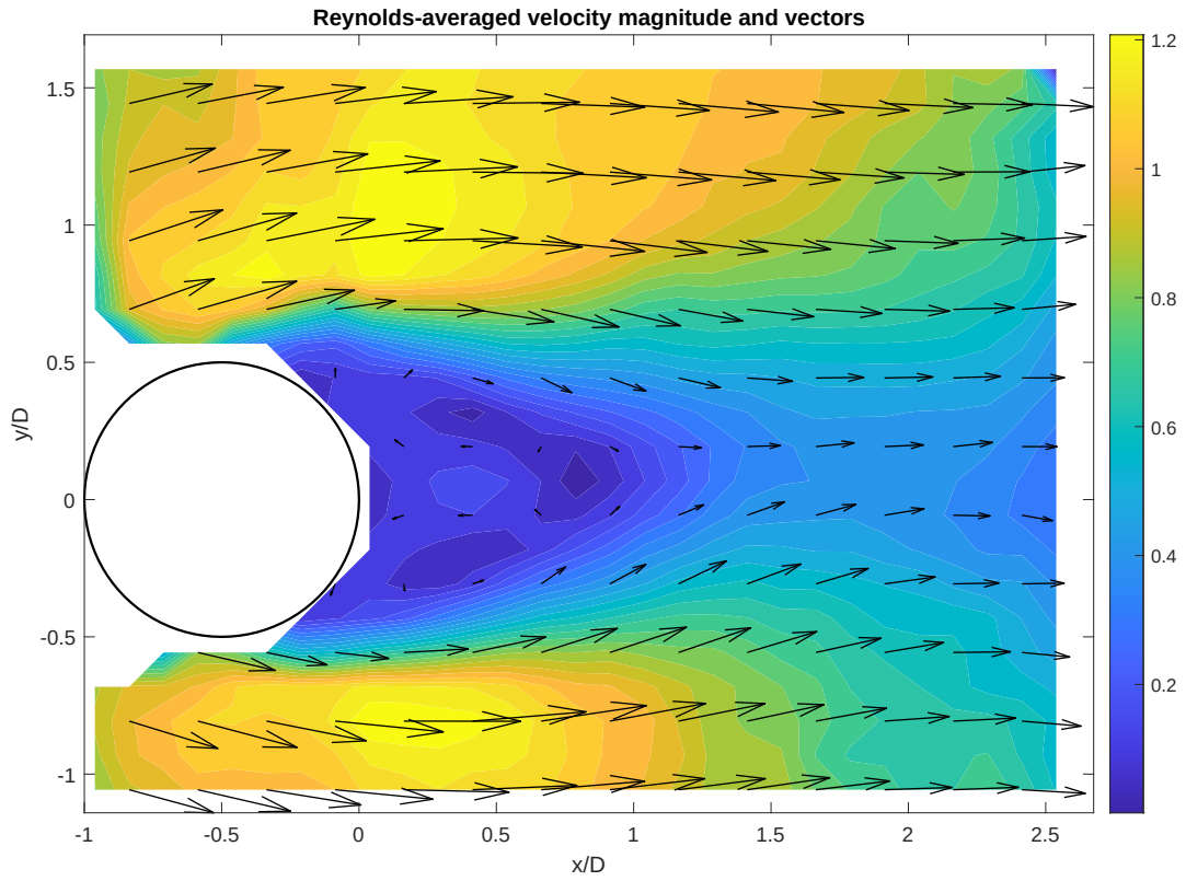
Figure 14: Mean dimensionless velocity magnitude and vectors at Re_D \simeq 9980 .
