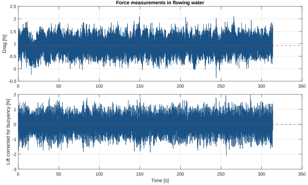
Figure 18: Drag and buoyancy-corrected lift in flowing water.
