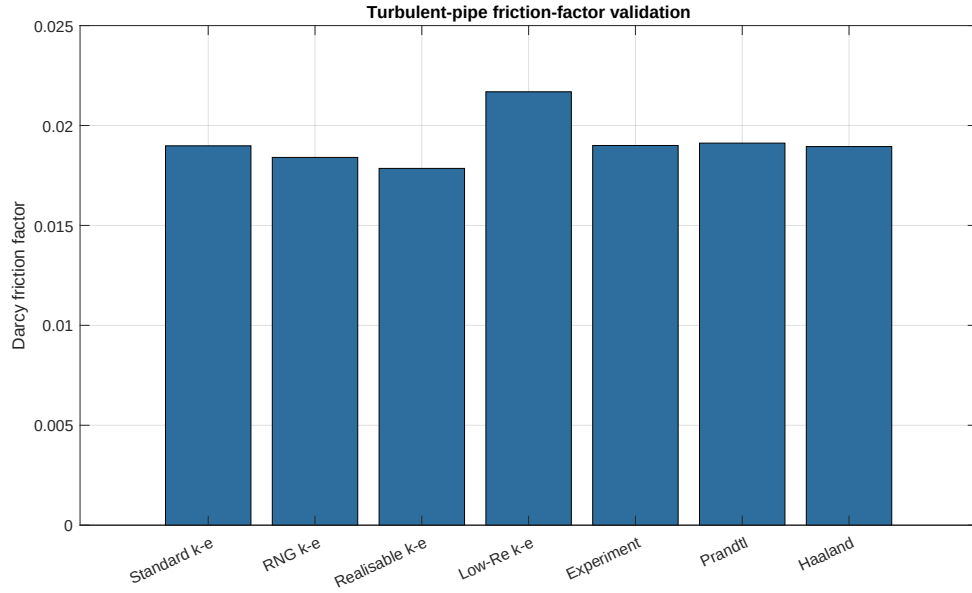
Figure 10: Darcy friction factors from the RANS solutions, experiment, and smooth-pipe correlations.
