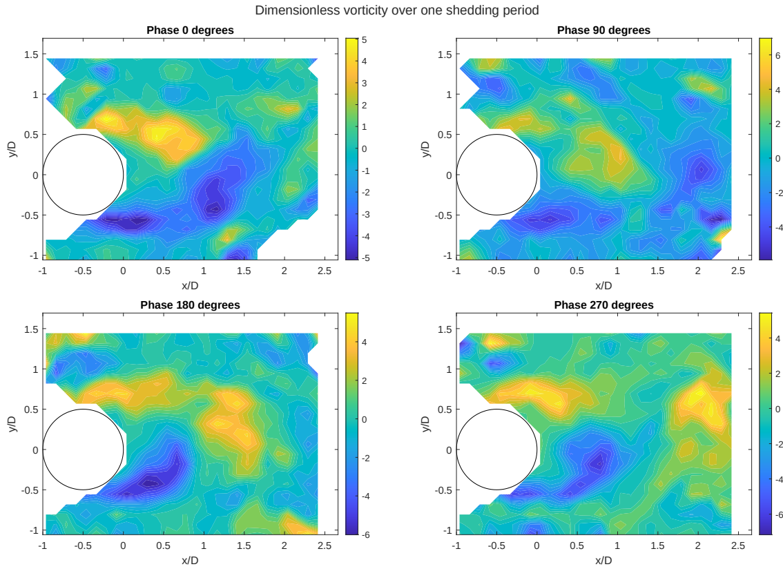
Figure 17: Dimensionless vorticity at four phases of one shedding period.
