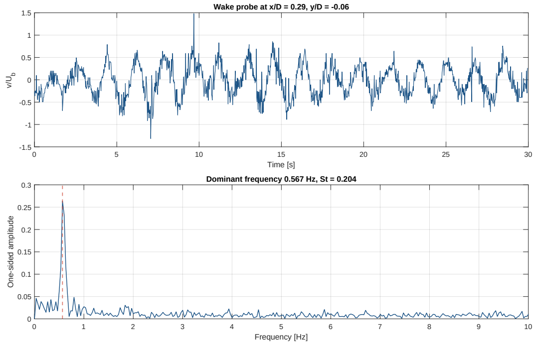
Figure 16: Transverse velocity at the wake probe and corresponding spectrum.
