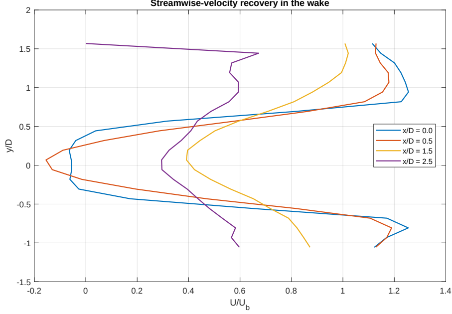
Figure 15: Recovery of the mean streamwise velocity at selected downstream positions.
