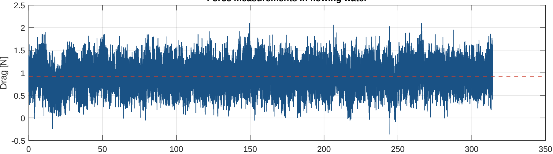
Force measurements in flowing water
