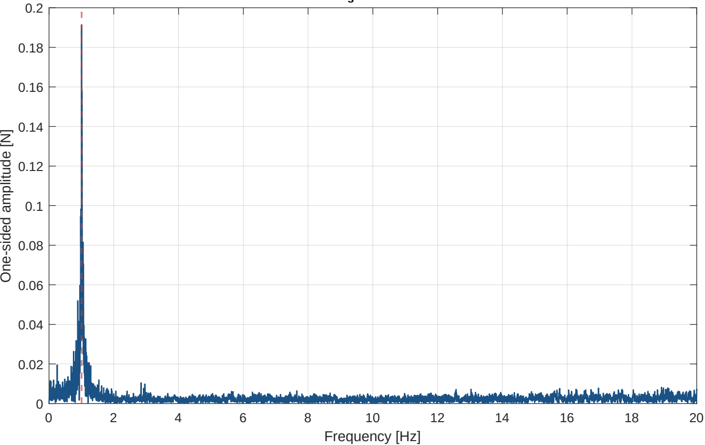
Lift spectrum: f_s = 1.006 Hz, St = 0.181
