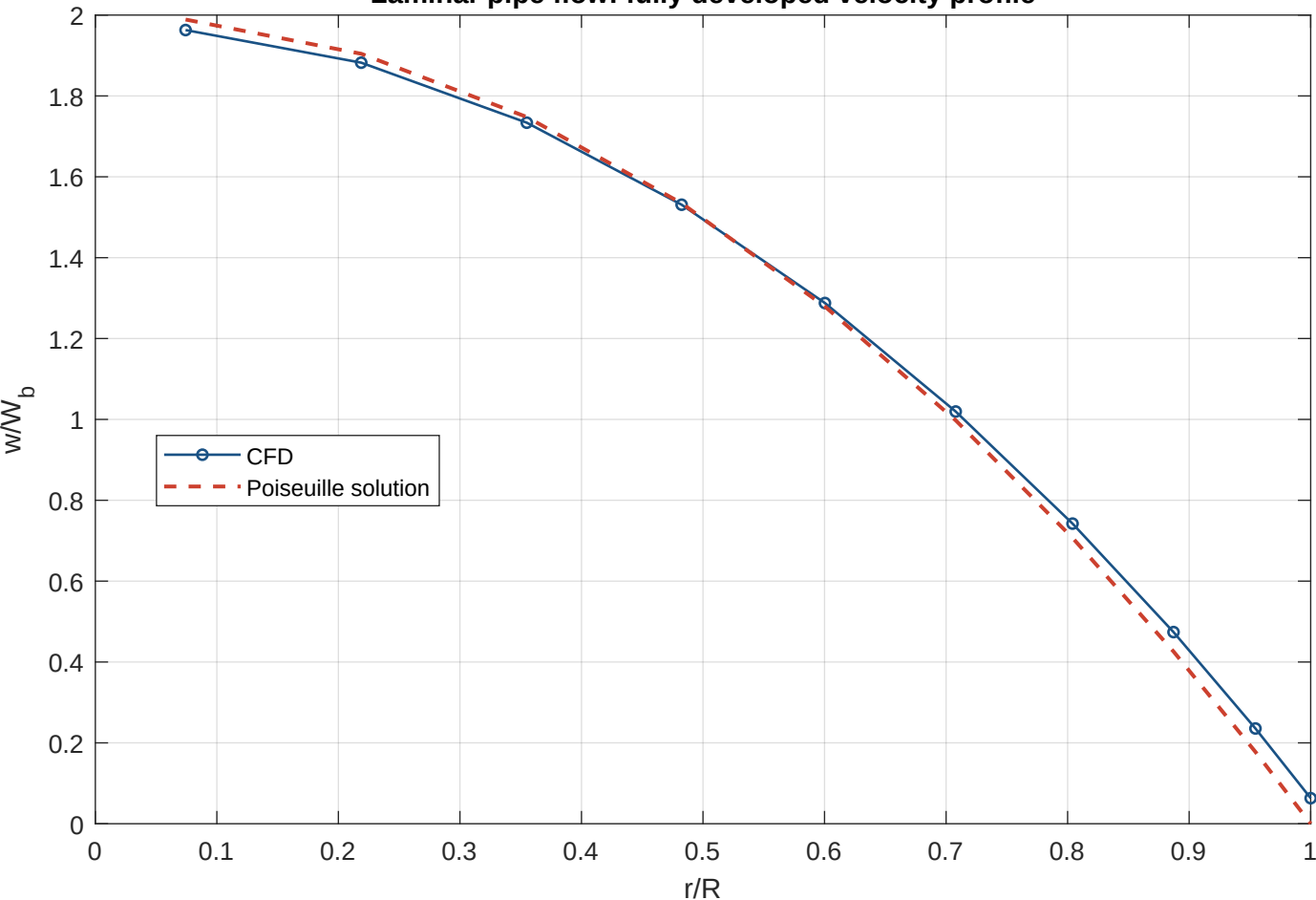
Laminar pipe flow: fully developed velocity profile
