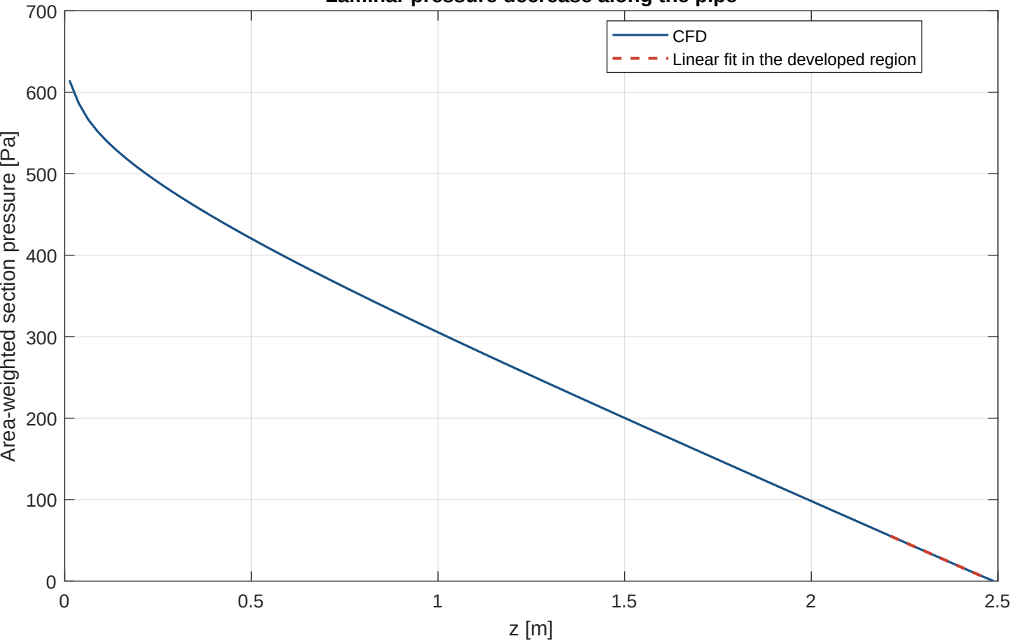
Laminar pressure decrease along the pipe
