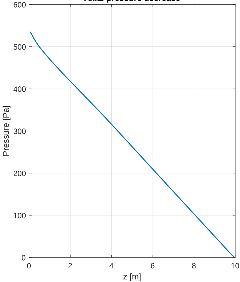
Axial pressure decrease
