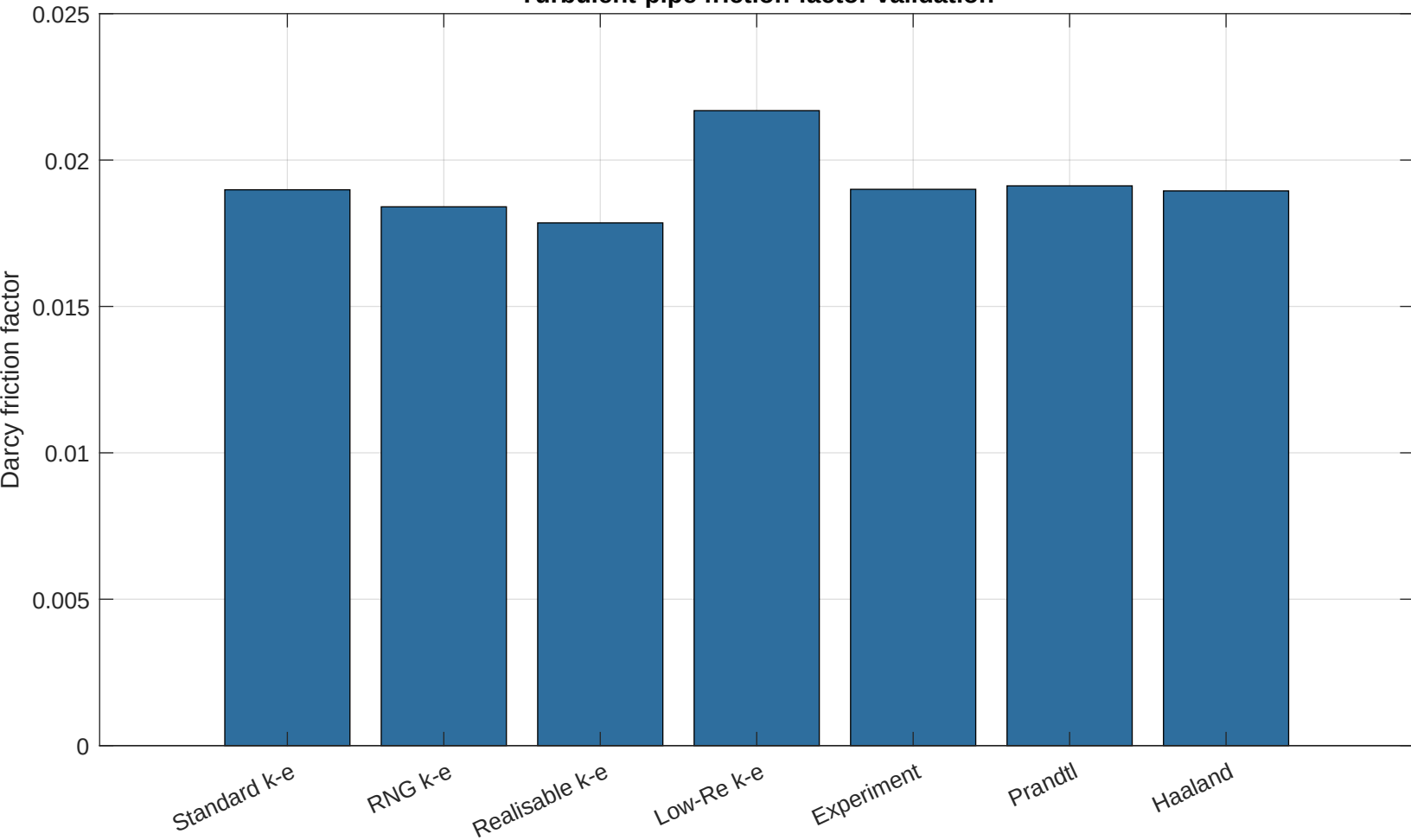
Turbulent-pipe friction-factor validation
