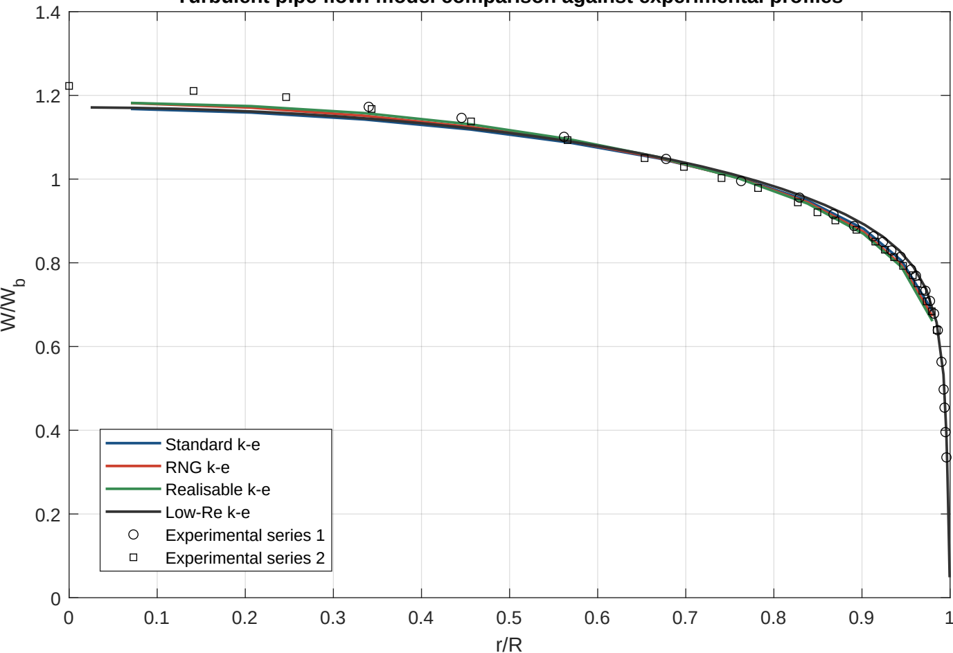
Turbulent pipe flow: model comparison against experimental profiles
