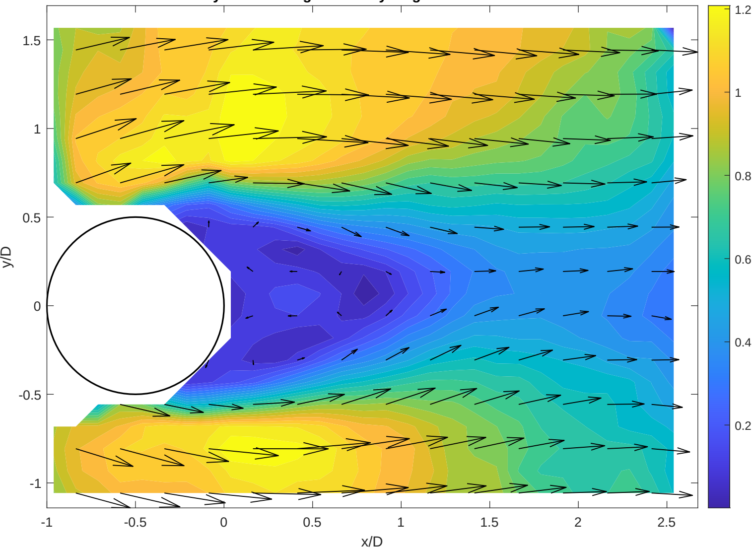
Reynolds-averaged velocity magnitude and vectors
