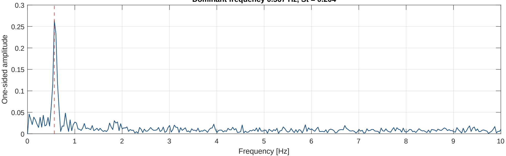
Dominant frequency 0.567 Hz, St = 0.204
