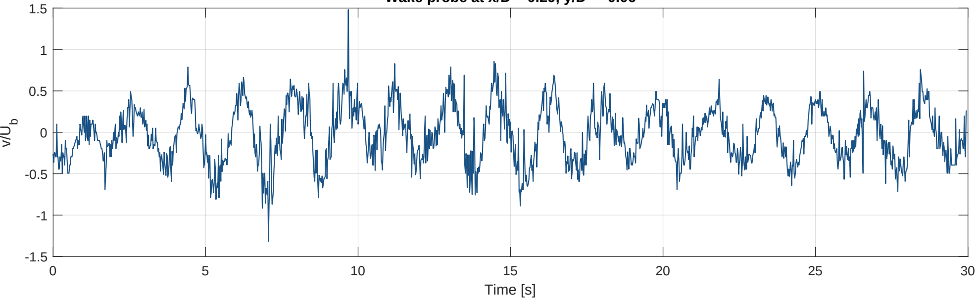
Dominant frequency 0.567 Hz, St = 0.204
