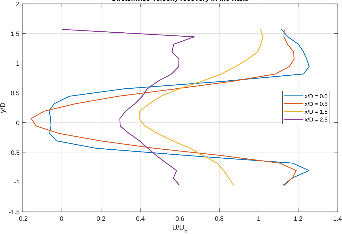
Stream-velocity recovery in the wake
