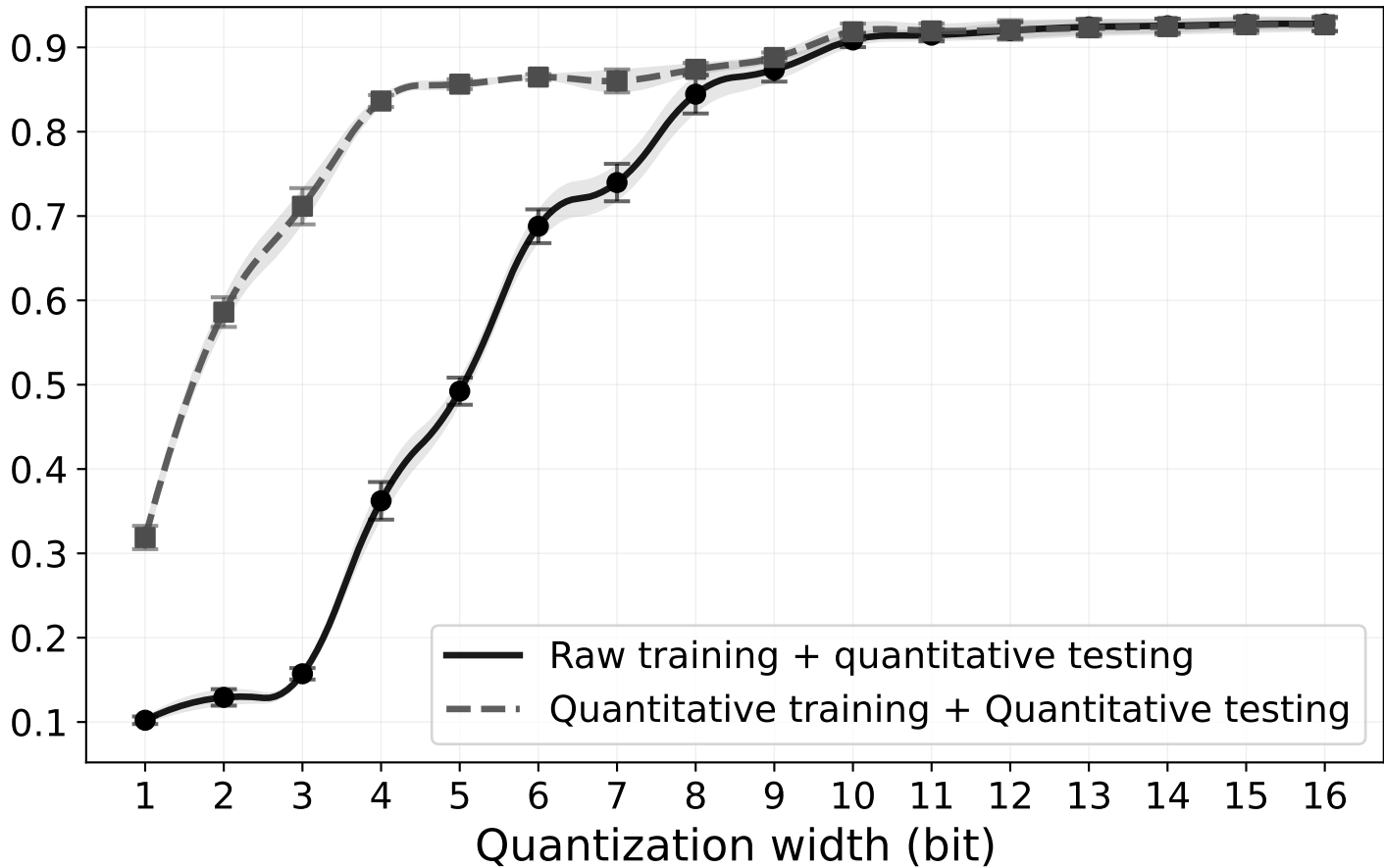
Macro F1-Score
