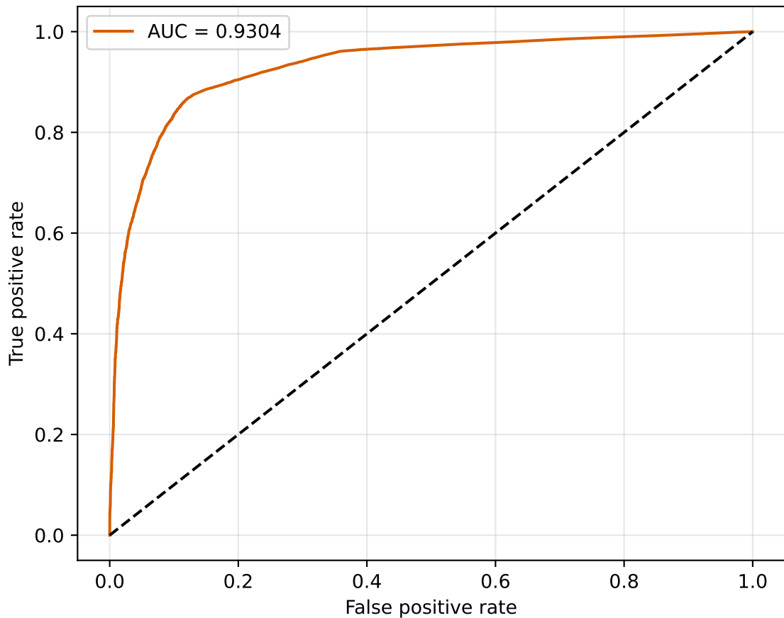
Best ROC from Sweep
