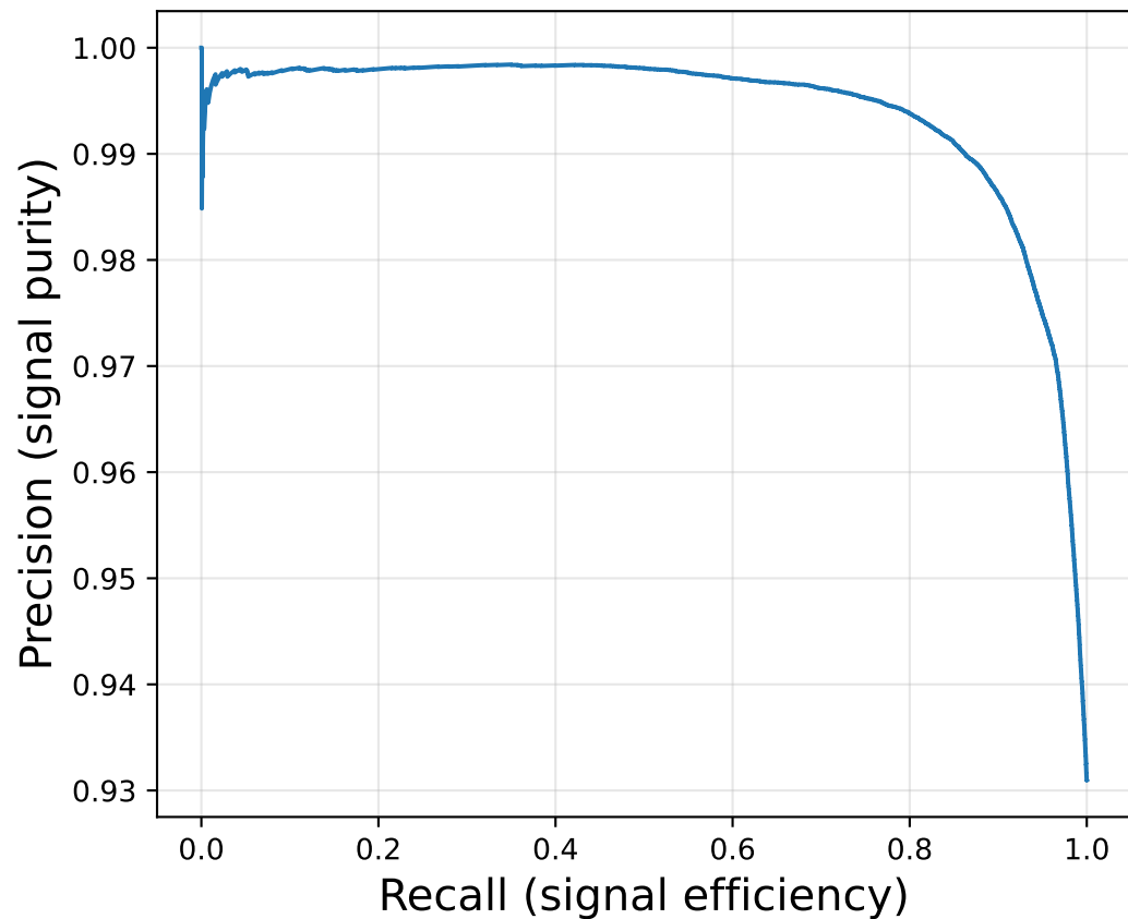
Precision-Recall Curve (AP=0.9941)
