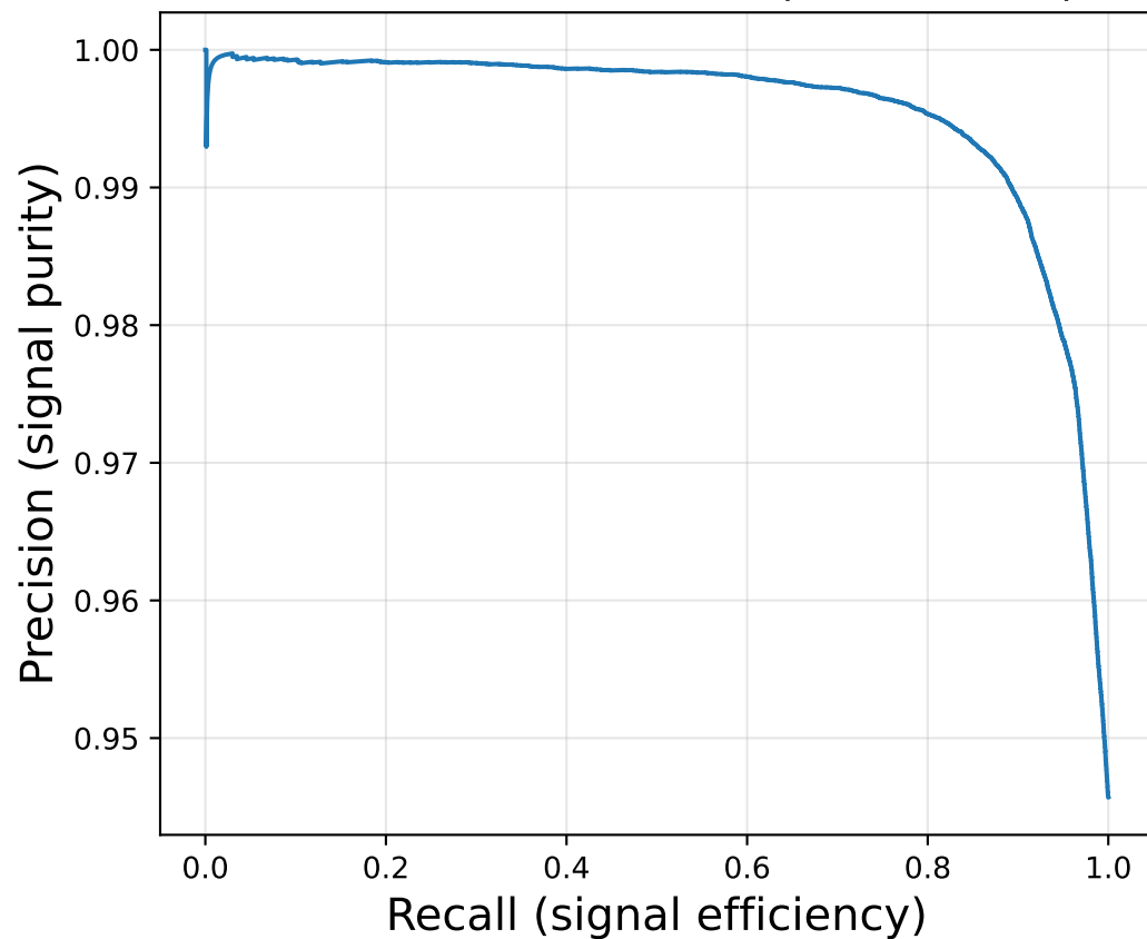
Precision-Recall Curve (AP=0.9955)
