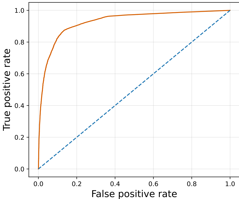
CNN ROC Curve
