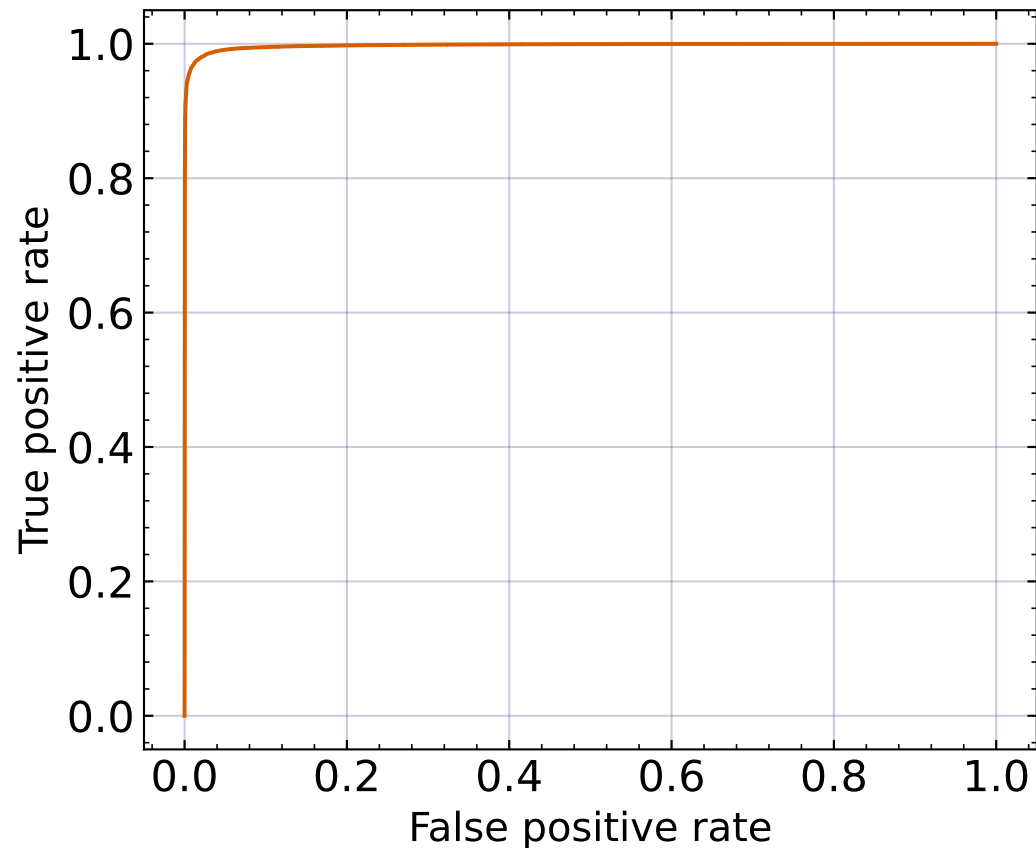
ROC curve
