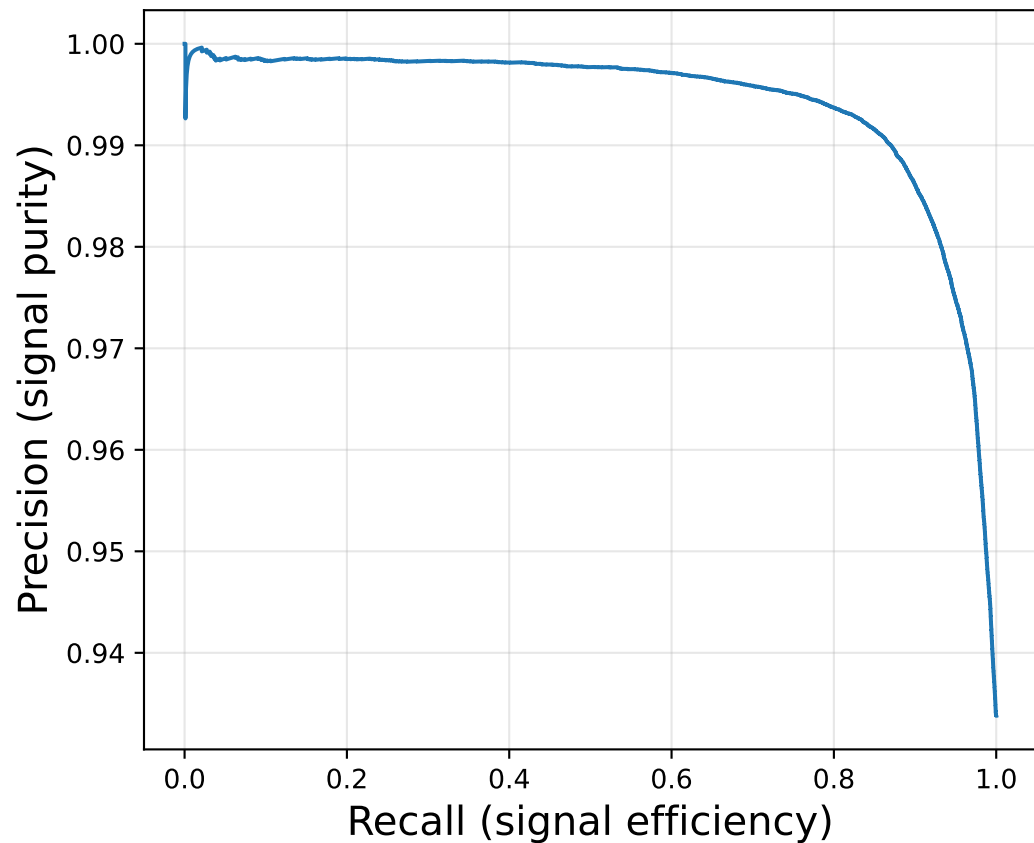
Precision-Recall Curve (AP=0.9942)
