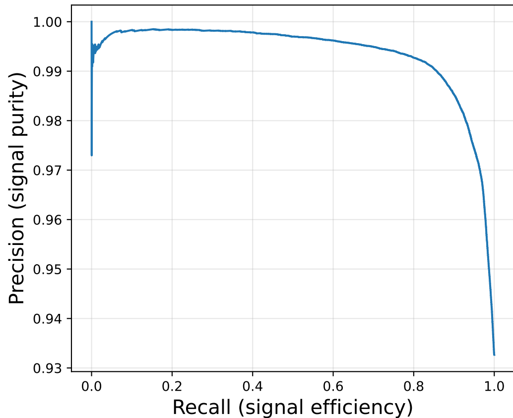
Precision-Recall Curve (AP=0.9935)
