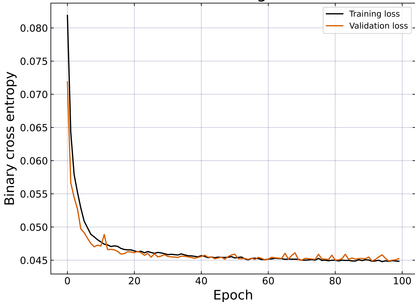
CNN training loss
