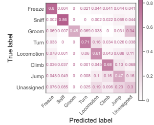
C Cross-validated confusion matrix
