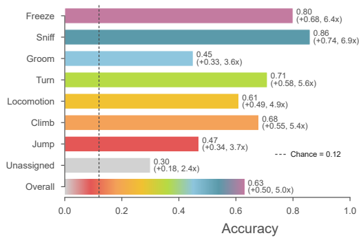
Accuracy versus chance
