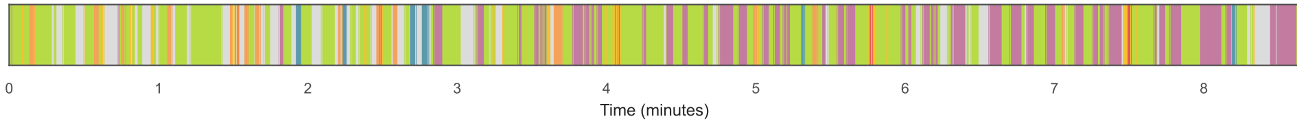
Behavioural barcode
