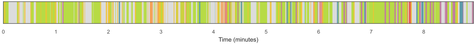
Behavioural barcode
