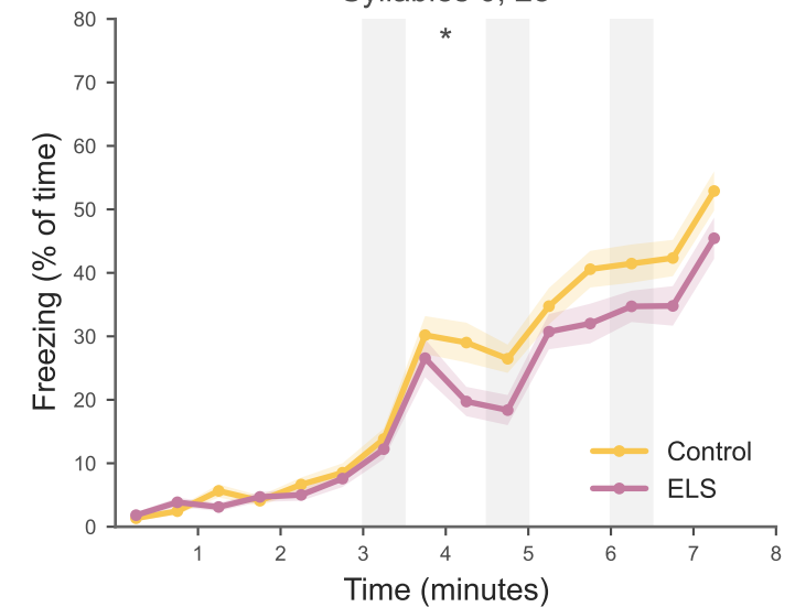
Syllables 0, 28
