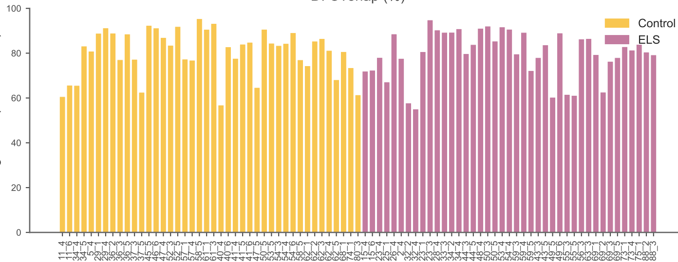
D. Overlap (%)
