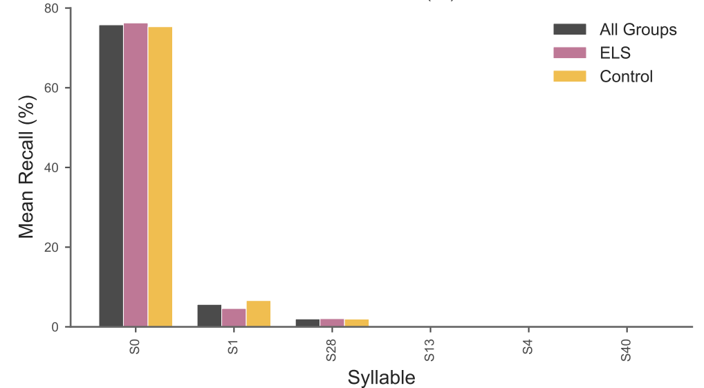
Syllables 0, 28
