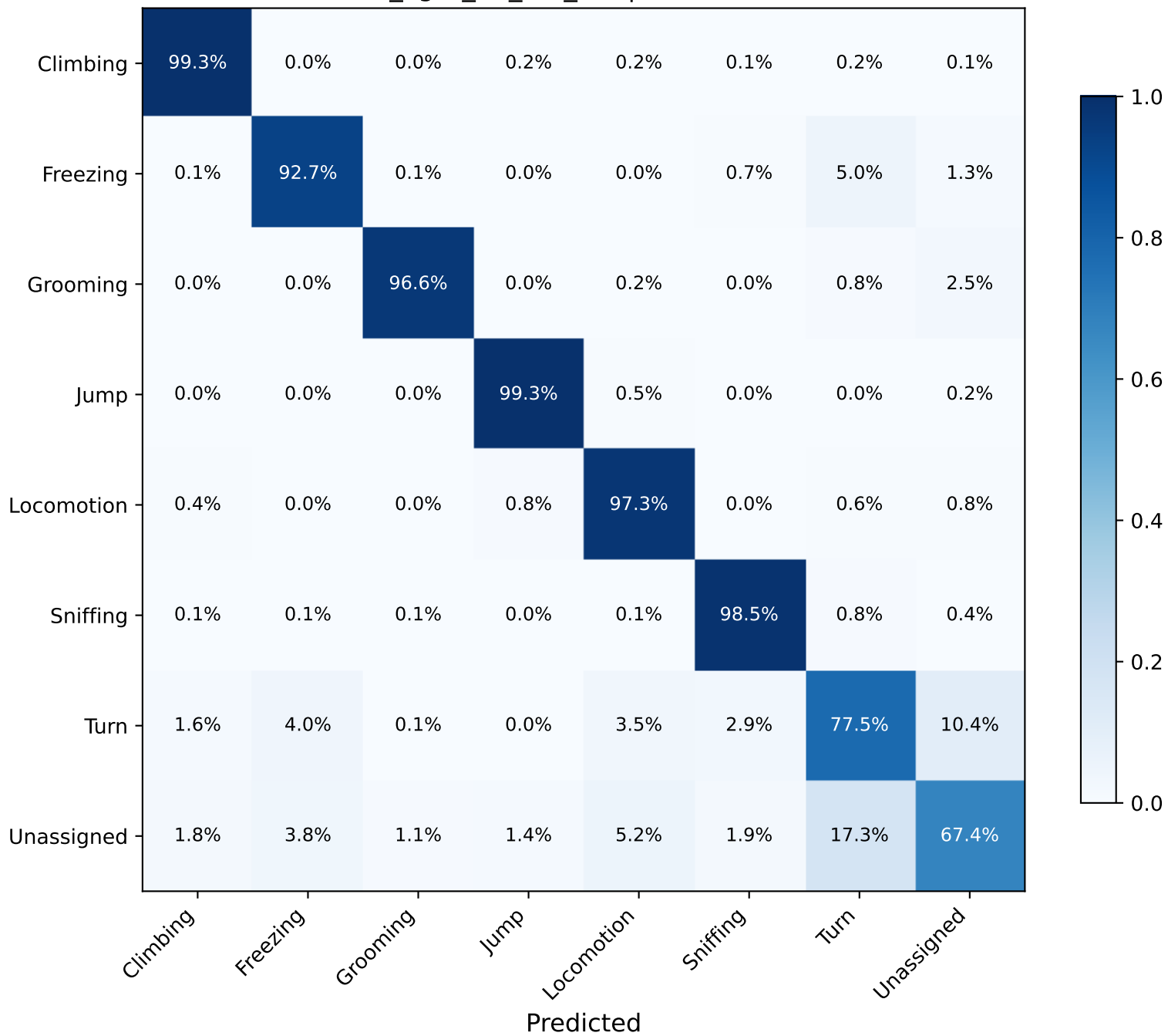
OOF Confusion Matrix (Row-Normalized) robust_light_no_tail_v2 | 0.903 macro F1
