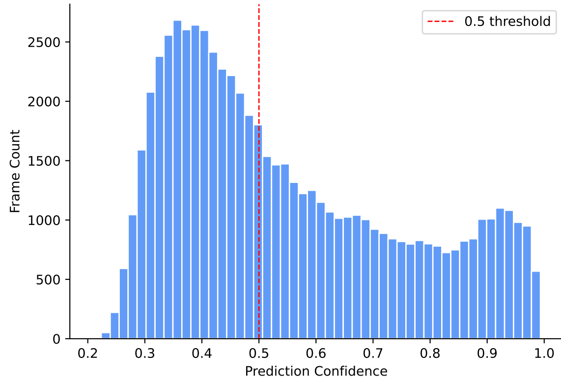
Overall Confidence (50.9% < 0.5)
