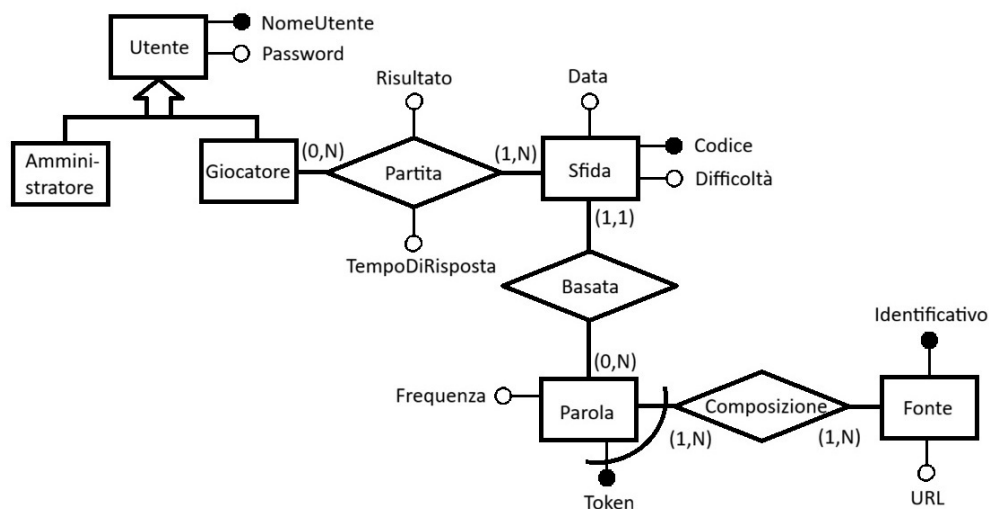
Schema E-R
