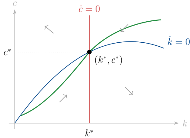
Figure 14: Phase diagram of the Ramsey-Cass-Koopmans model. The equilibrium (k^*, c^*) is a saddle point. The gray arrows show the direction of motion in each region; only the green trajectory (stable branch) converges to the equilibrium.
