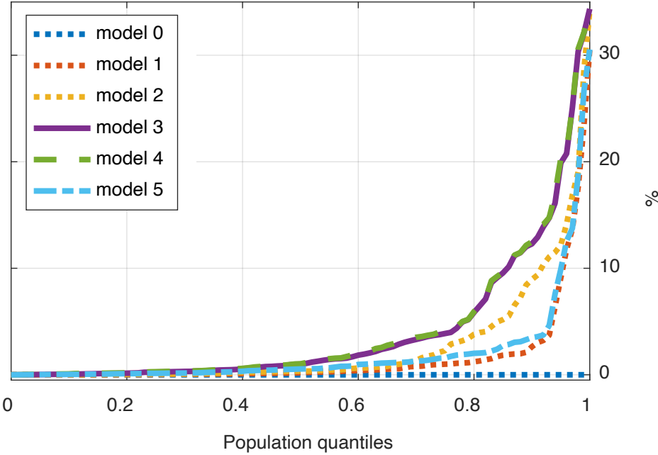
Absolute deviance explained
