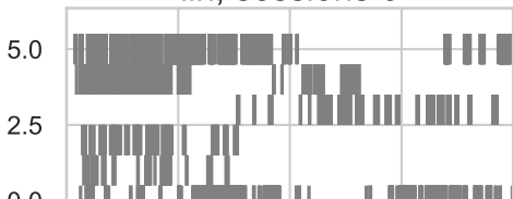
lin, sessions 6
