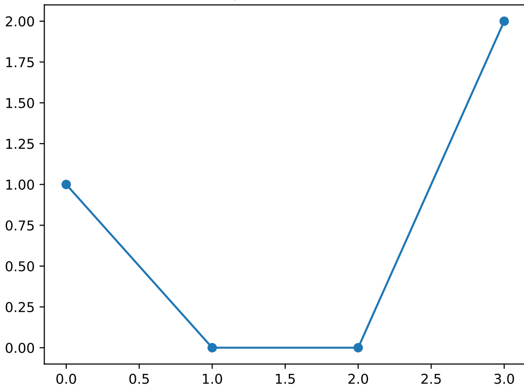
Shapelet number 33
