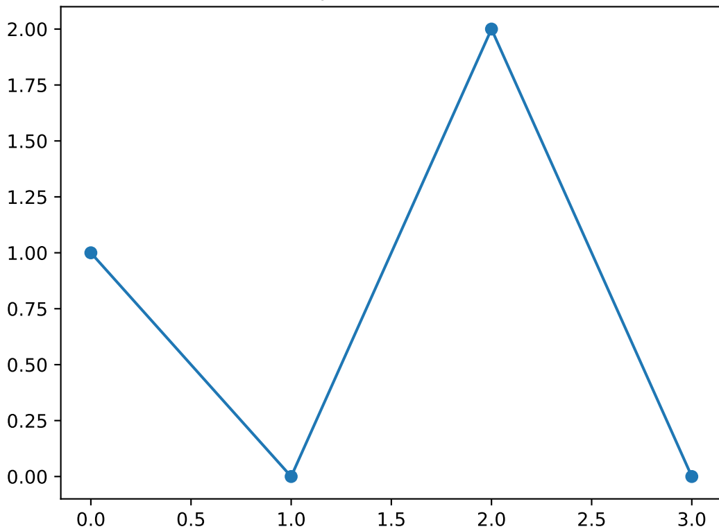
Shapelet number 35
