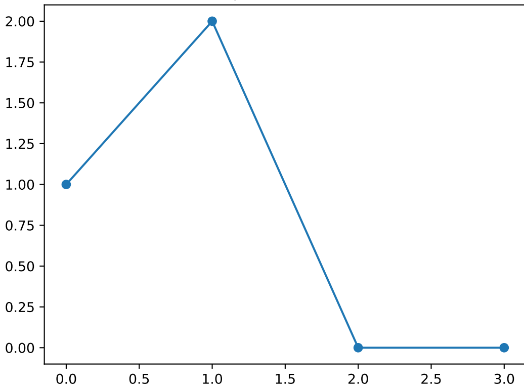
Shapelet number 40
