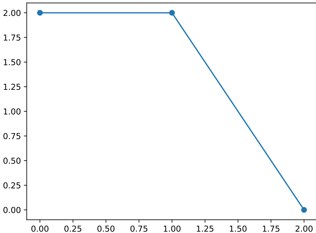
Shapelet number 13
