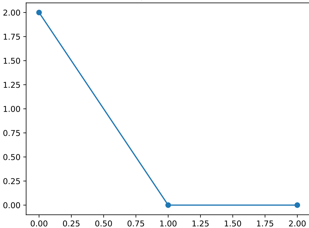
Shapelet number 9
