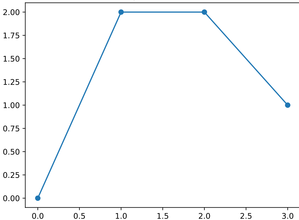
Shapelet number 31
