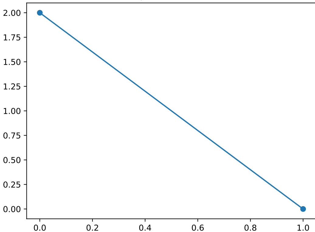
Shapelet number 16
