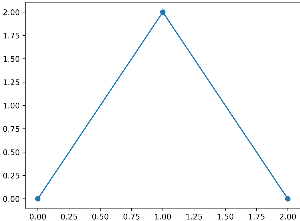
Shapelet number 4
