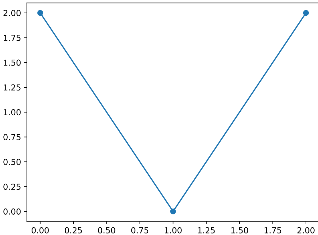
Shapelet number 11
