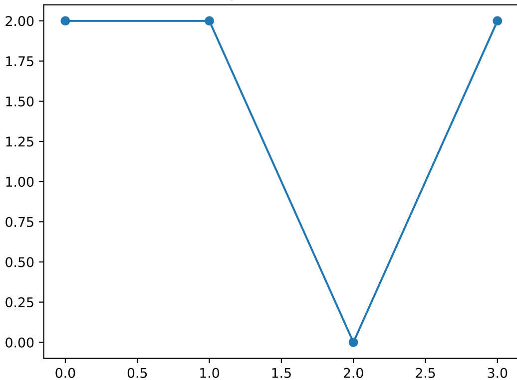
Shapelet number 61
