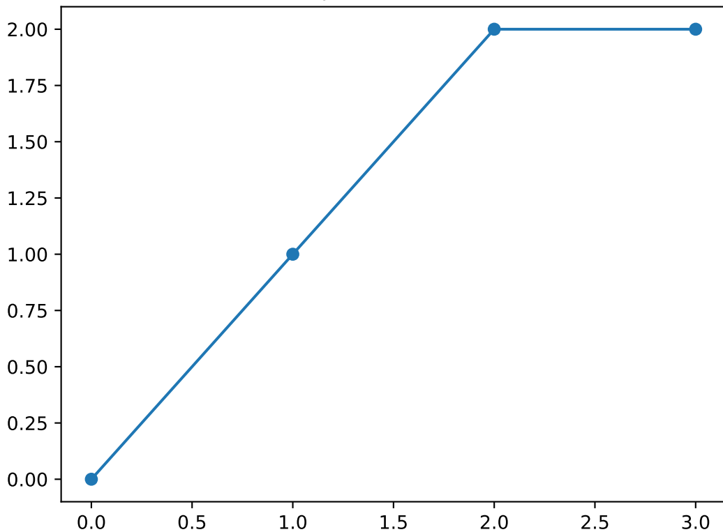
Shapelet number 24
