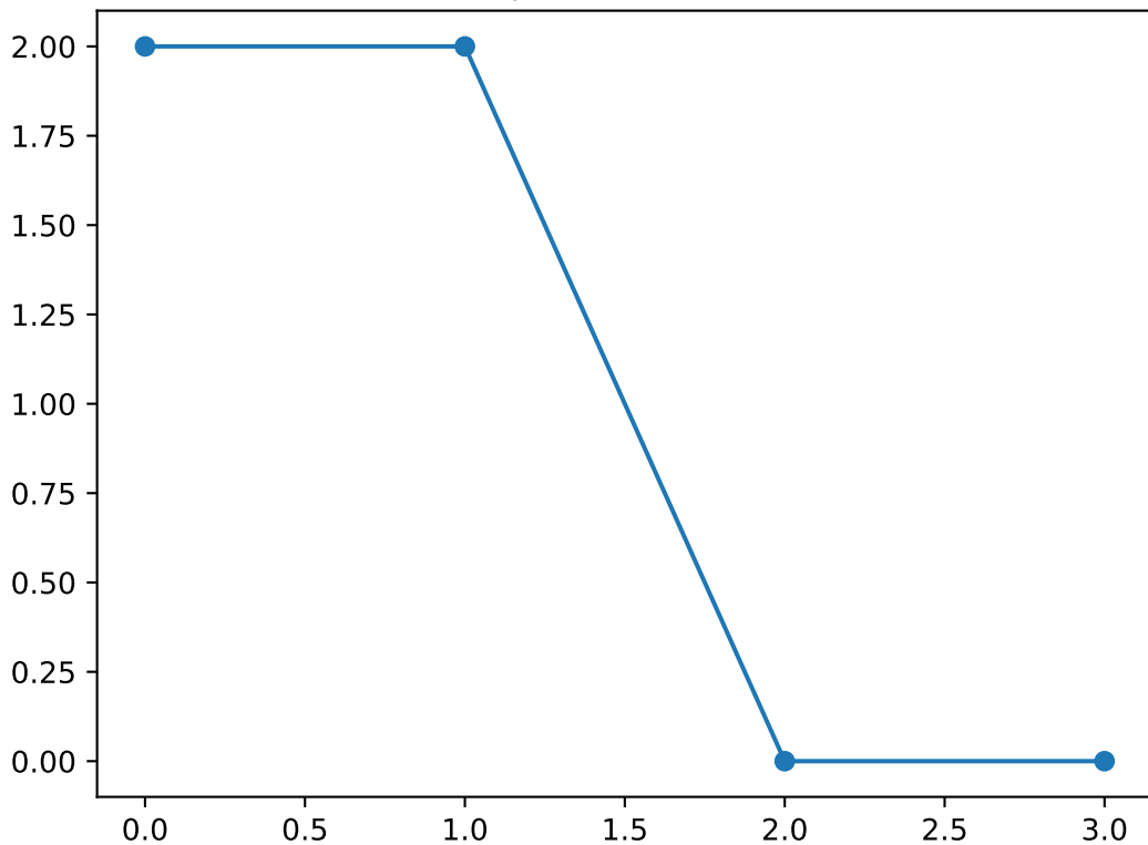
Shapelet number 66
