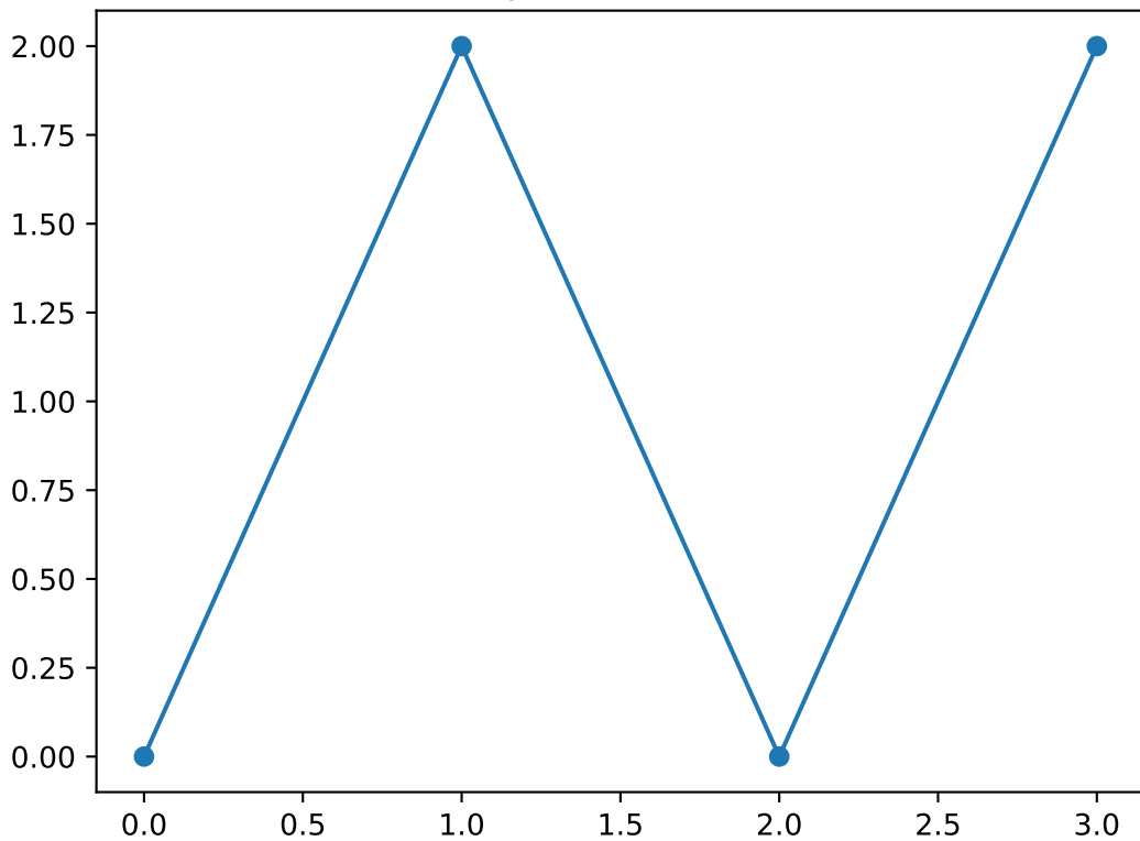
Shapelet number 26
