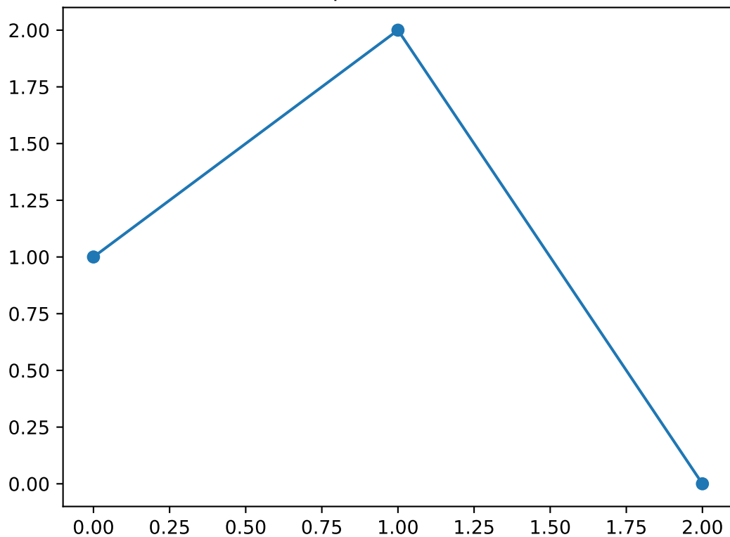
Shapelet number 8
