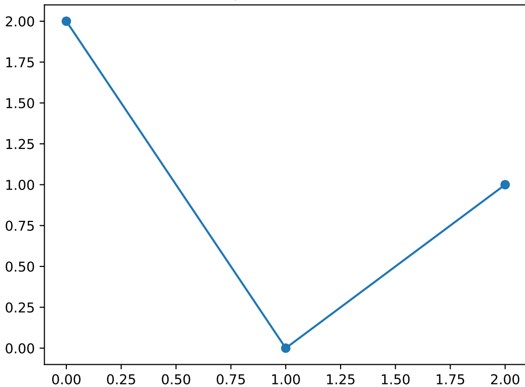
Shapelet number 10
