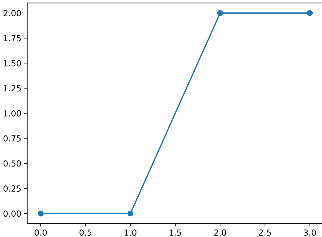
Shapelet number 19
