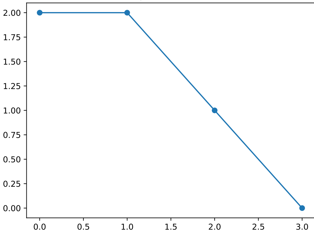
Shapelet number 68
