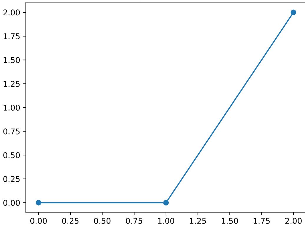
Shapelet number 2
