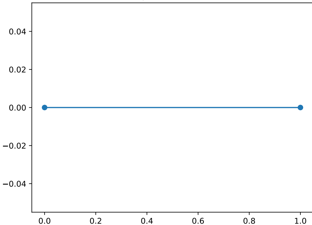
Shapelet number 16
