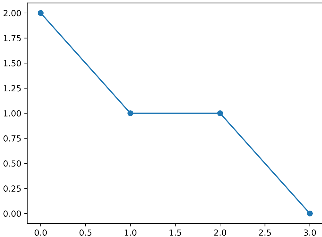
Shapelet number 64
