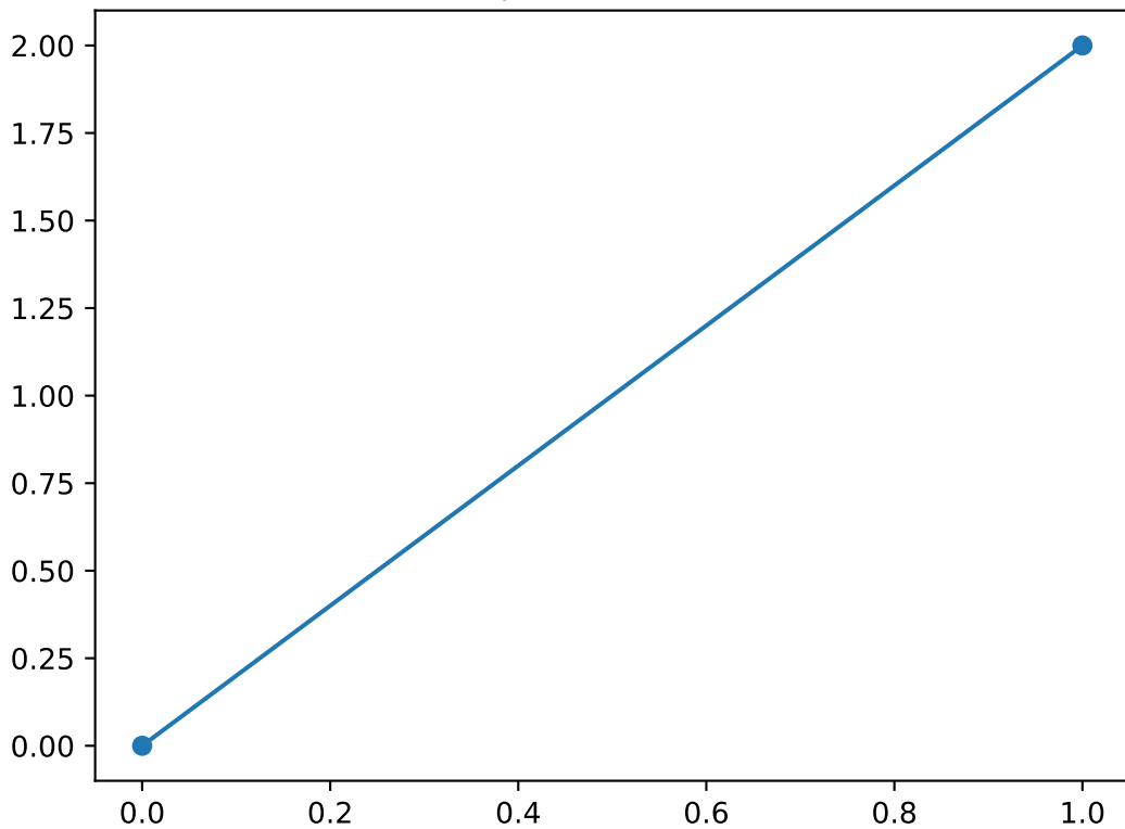
Shapelet number 14
