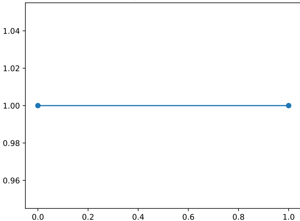
Shapelet number 15
