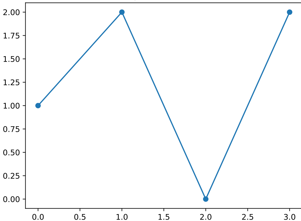
Shapelet number 42
