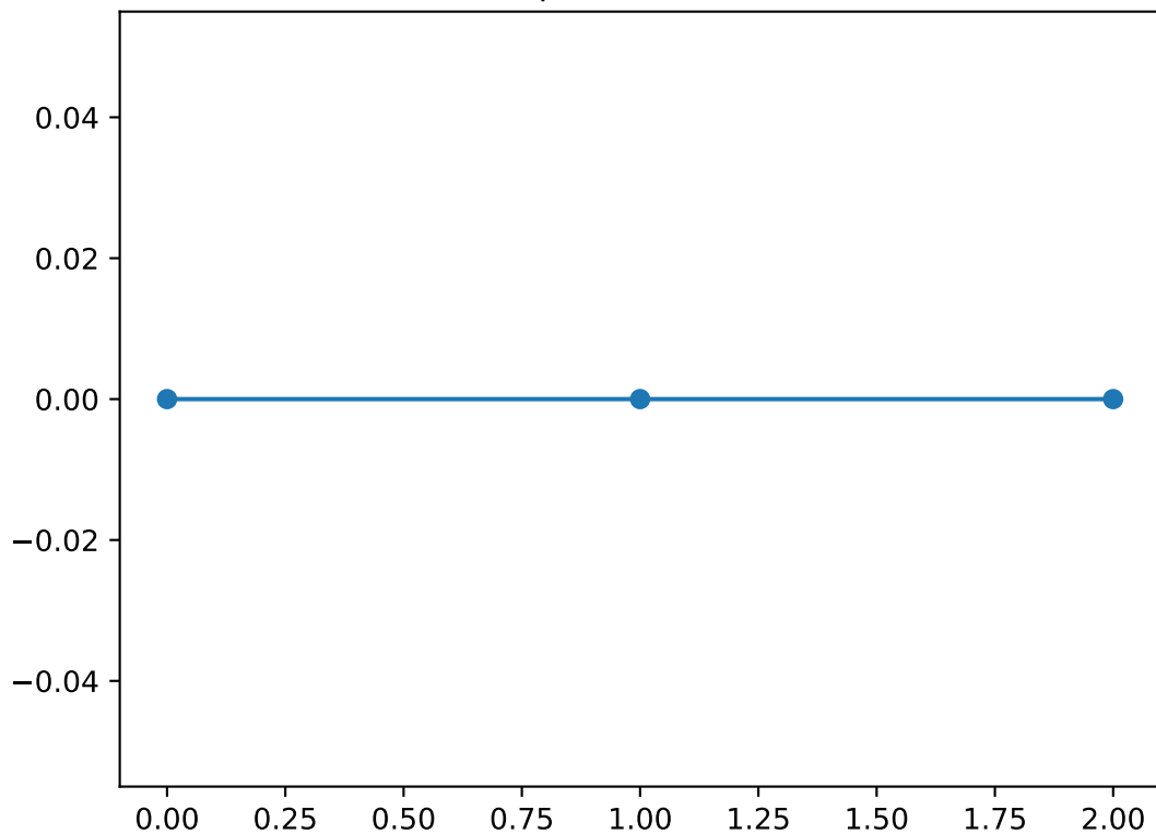
Shapelet number 3
