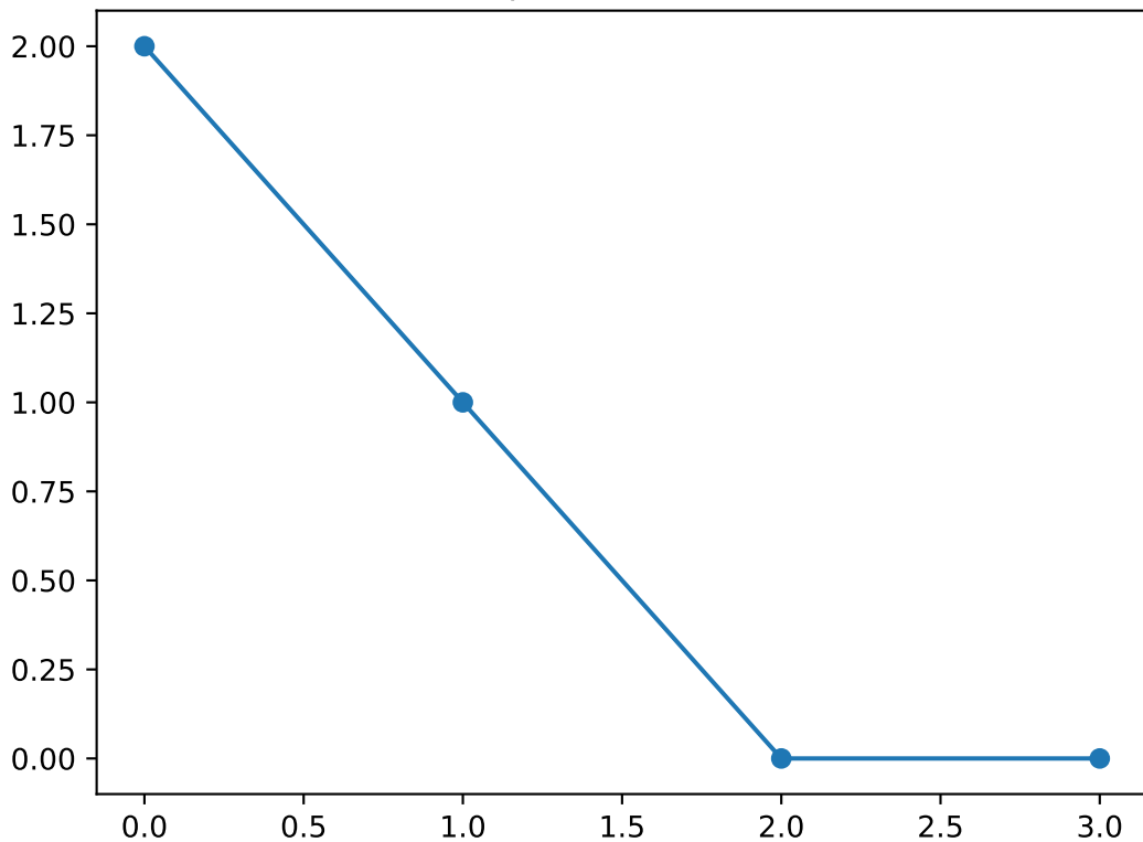
Shapelet number 54
