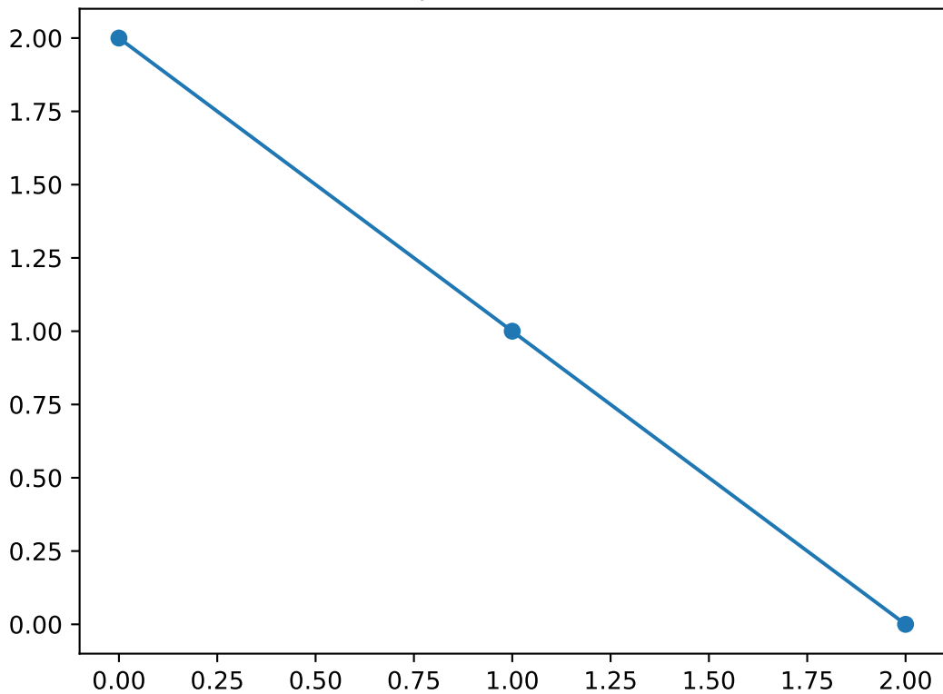
Shapelet number 12
