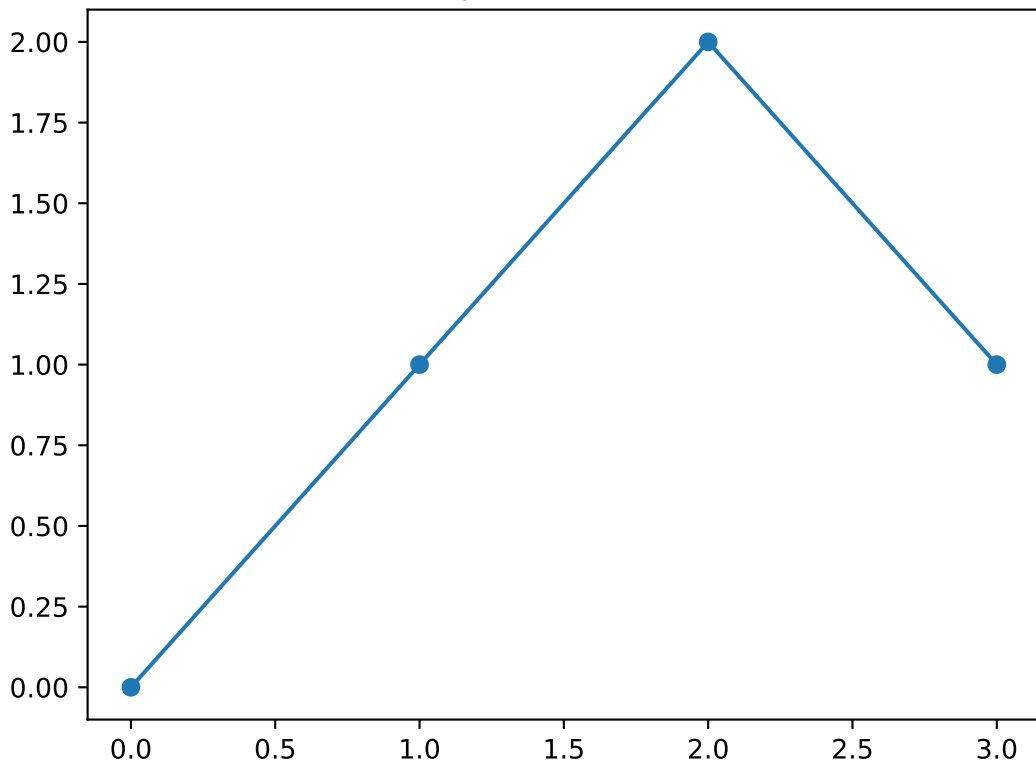
Shapelet number 23
