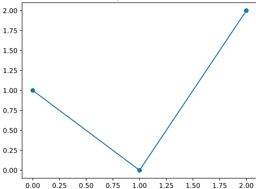
Shapelet number 9
