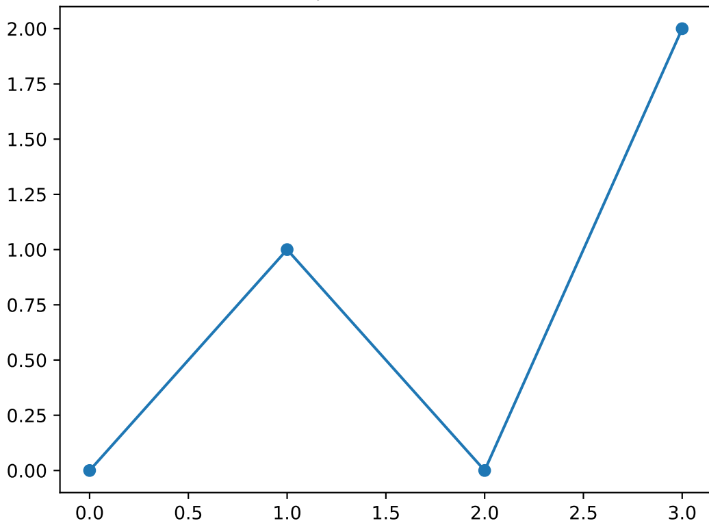
Shapelet number 20
