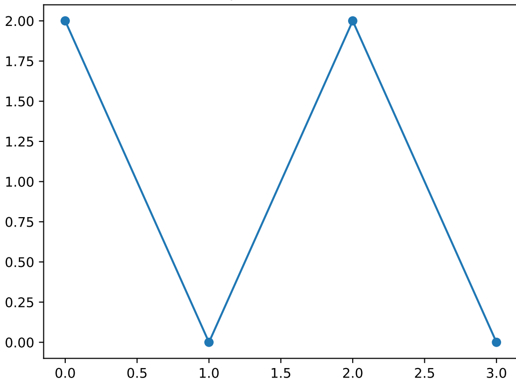
Shapelet number 51
