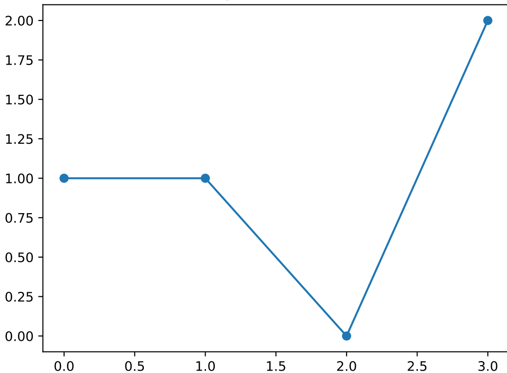
Shapelet number 38
