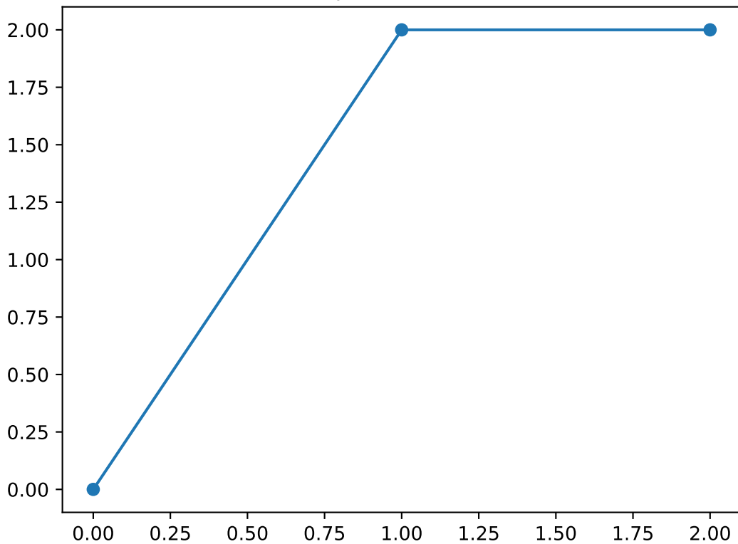
Shapelet number 8
