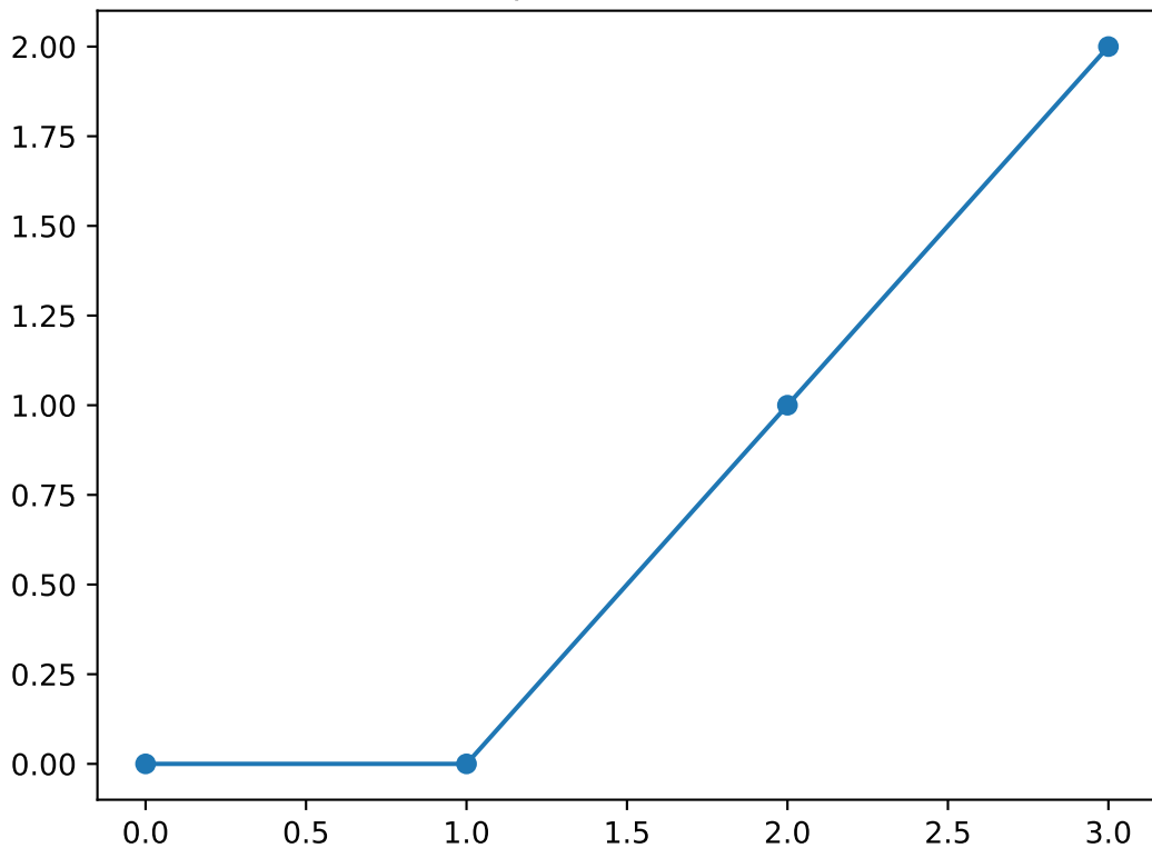
Shapelet number 17
