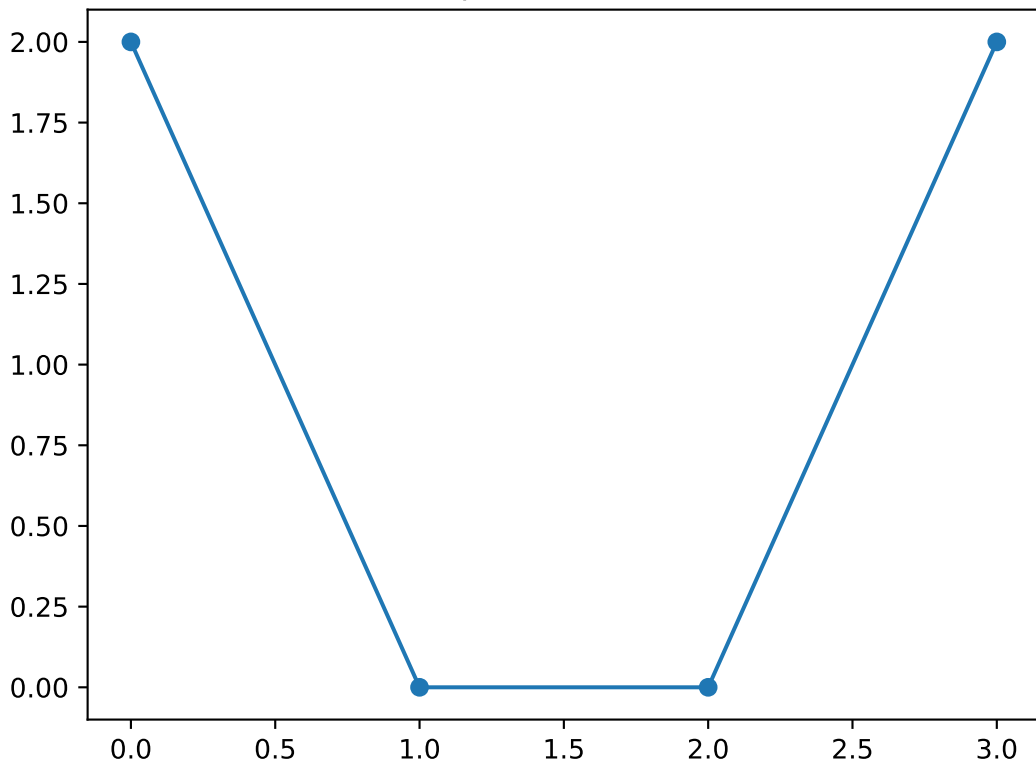
Shapelet number 47
