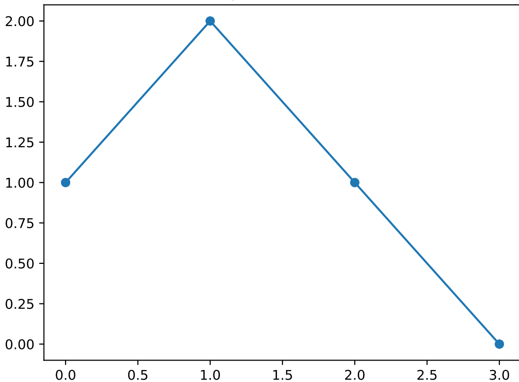
Shapelet number 43
