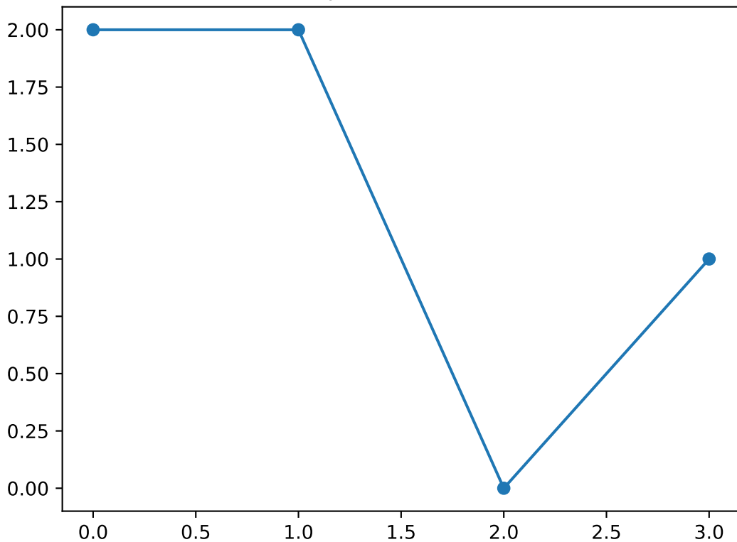
Shapelet number 67
