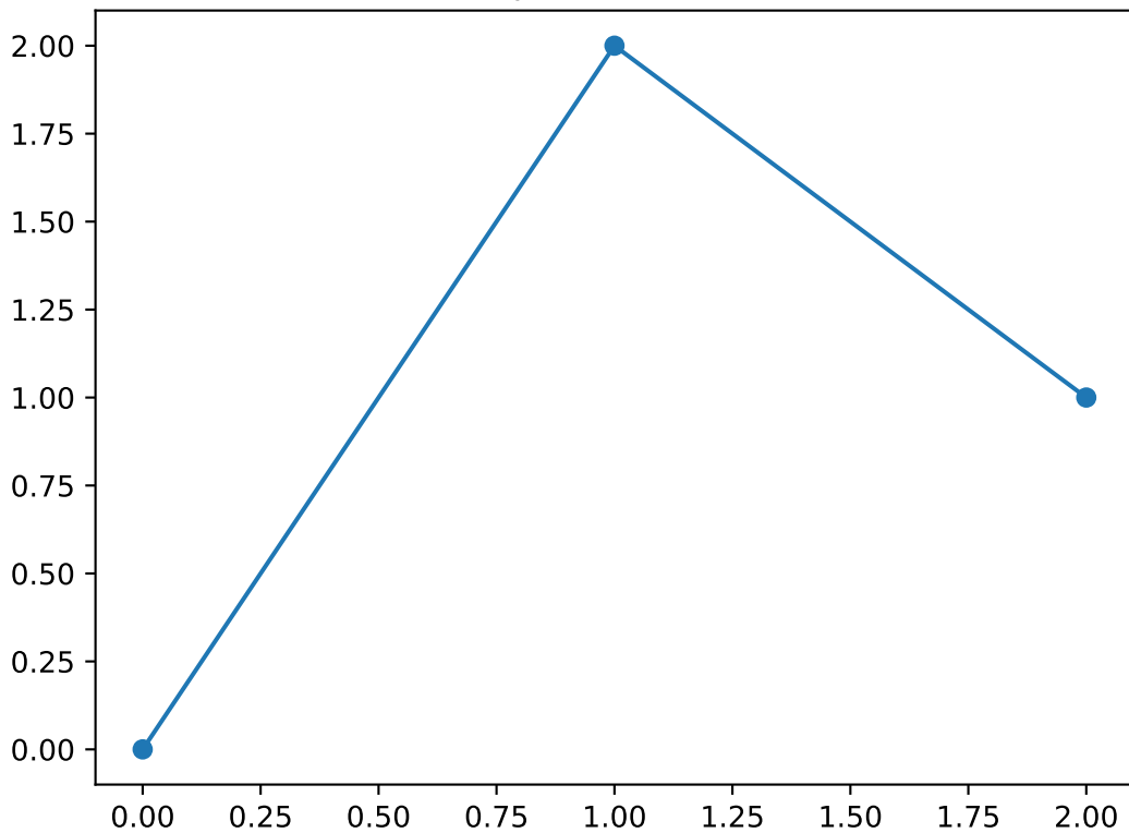
Shapelet number 5
