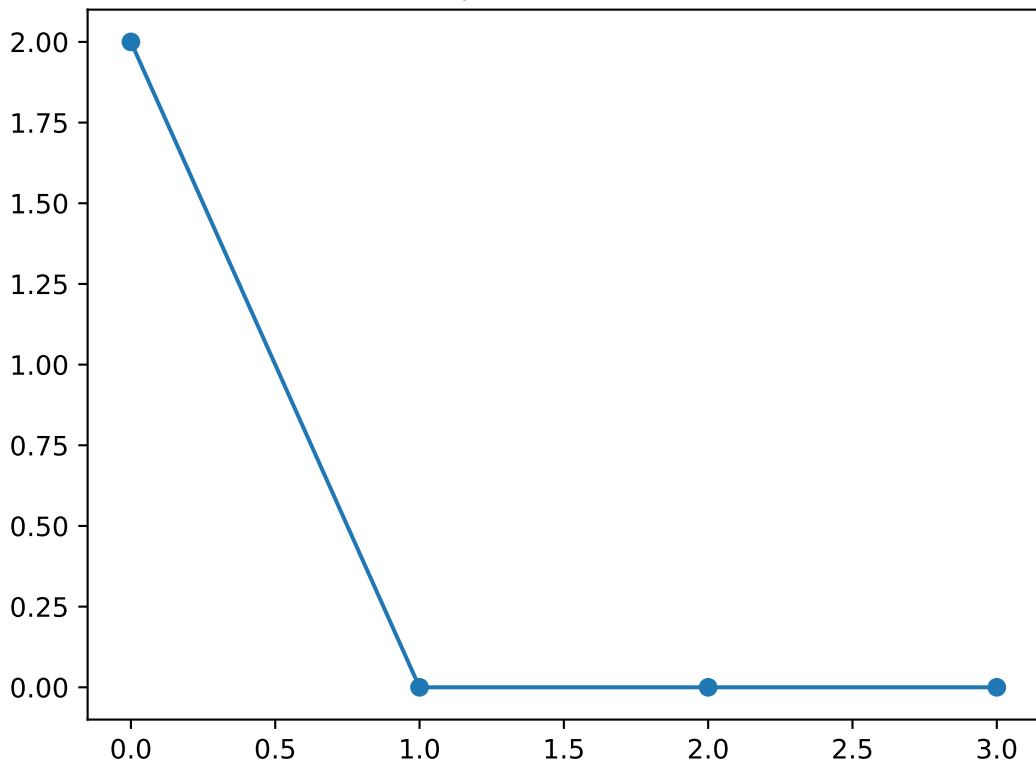
Shapelet number 45
