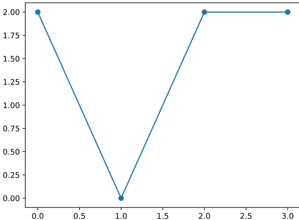
Shapelet number 53
