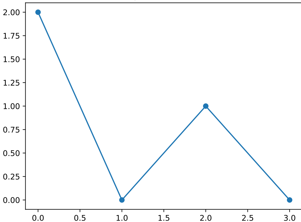
Shapelet number 48
