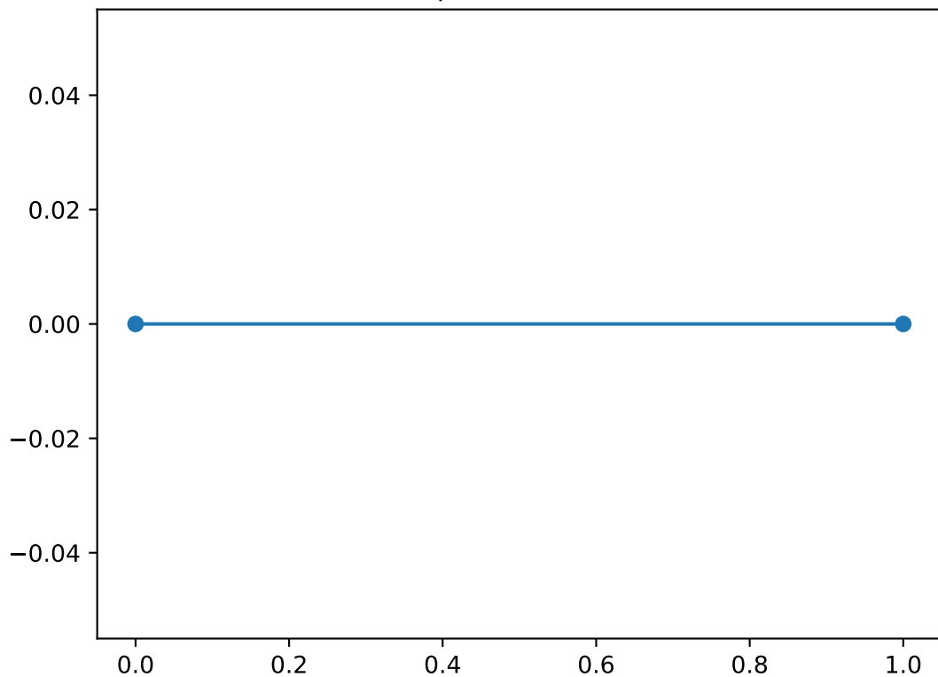
Shapelet number 0
