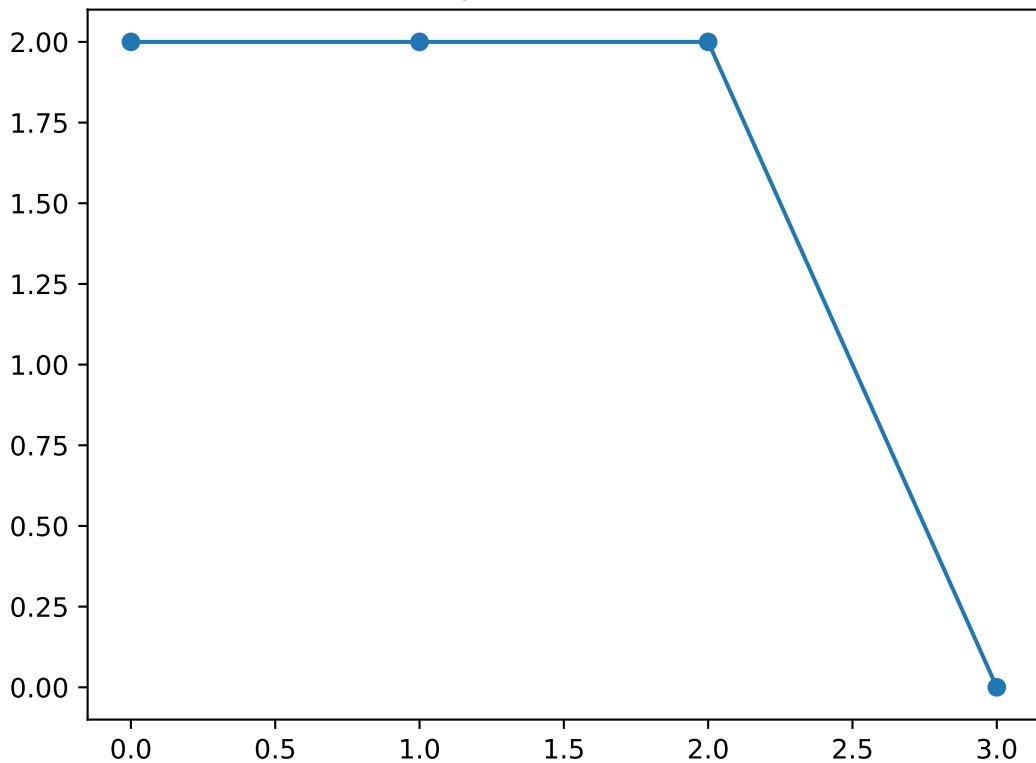
Shapelet number 63
