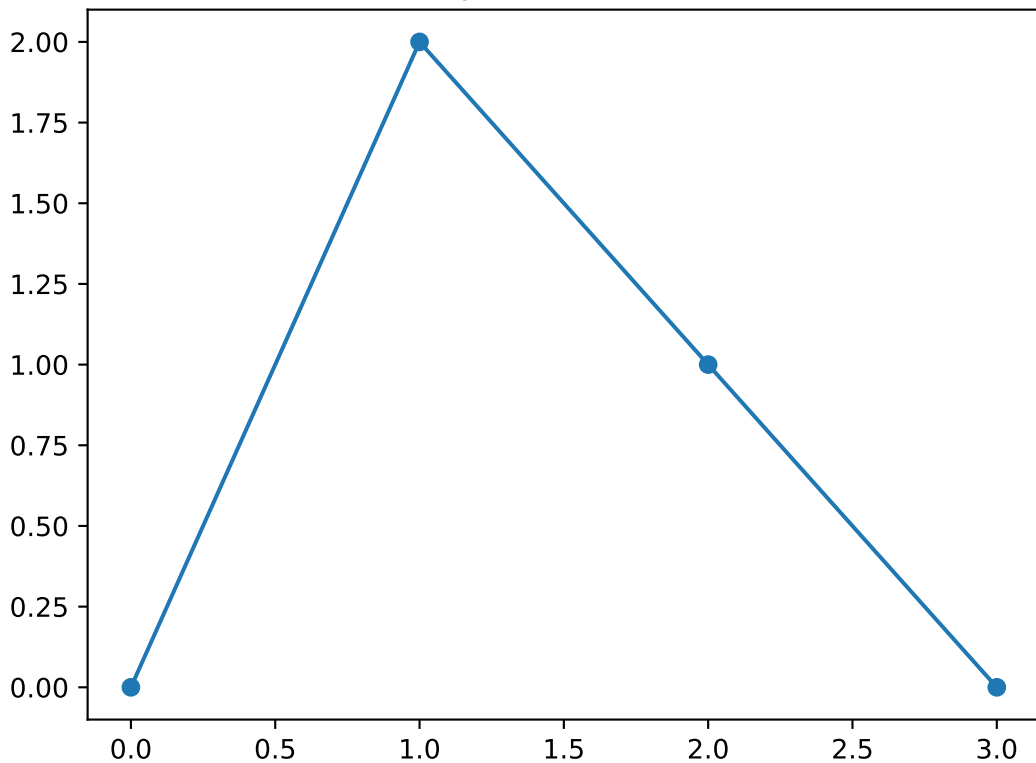
Shapelet number 27
