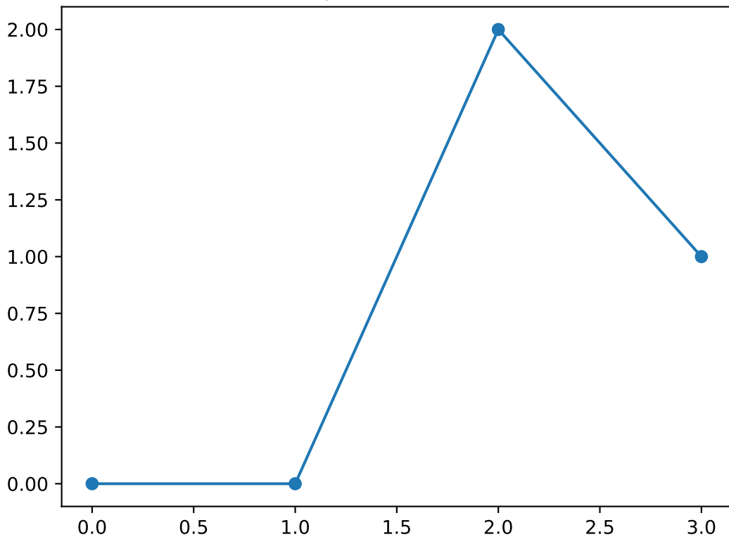
Shapelet number 18
