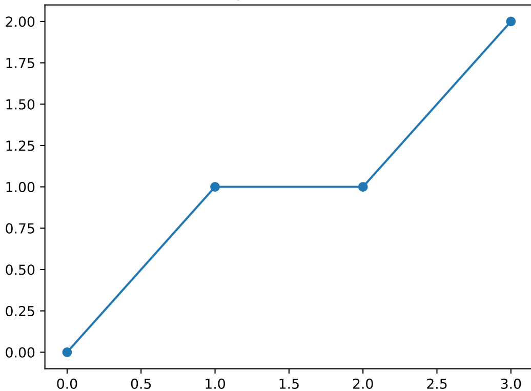
Shapelet number 21
