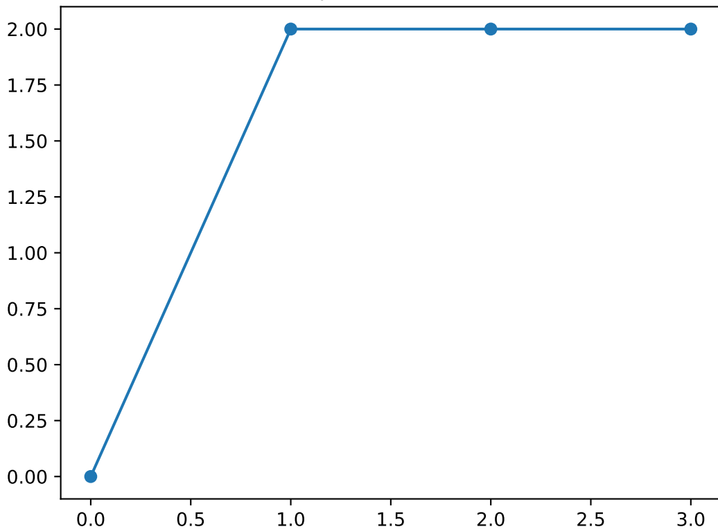
Shapelet number 32
