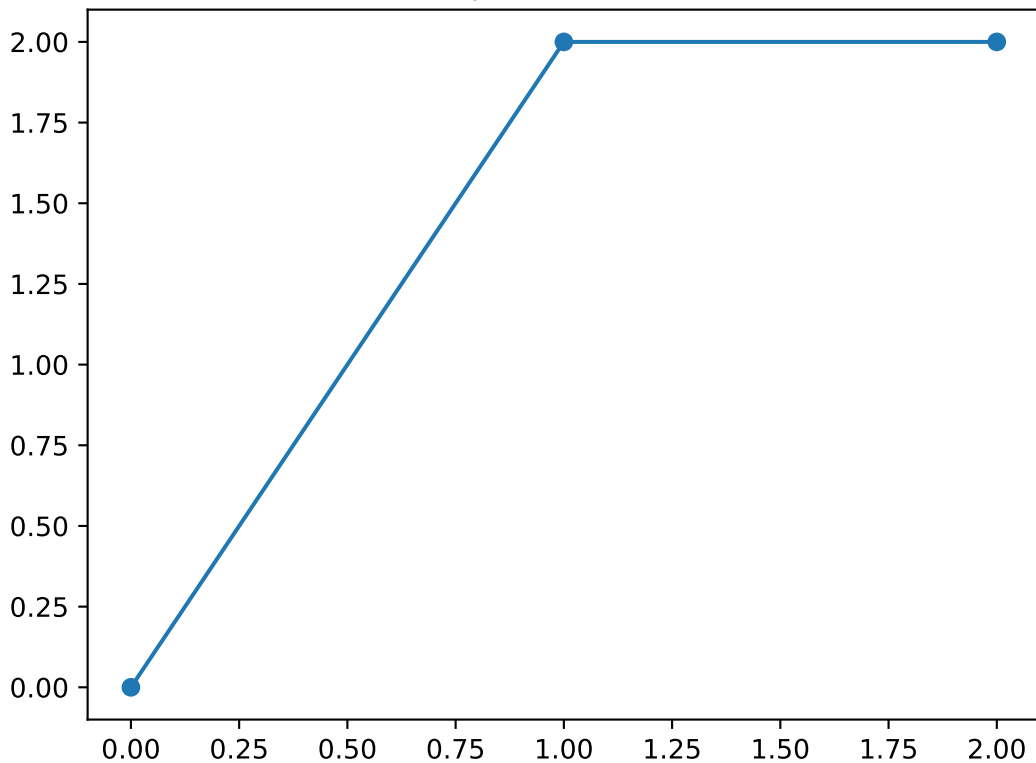
Shapelet number 6
