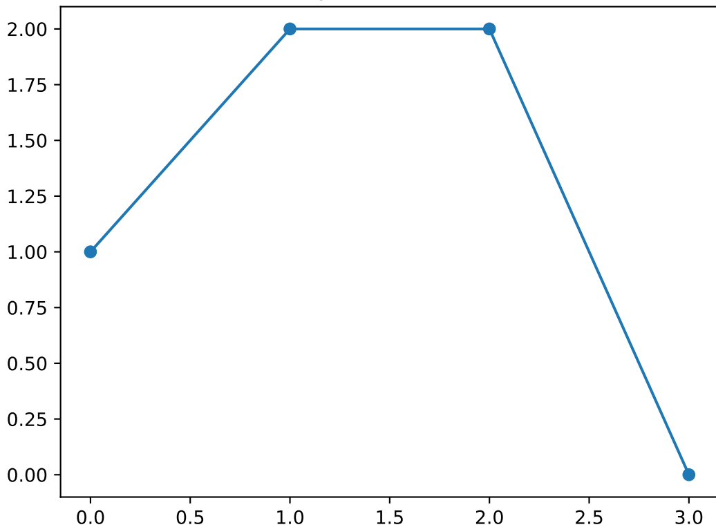
Shapelet number 44
