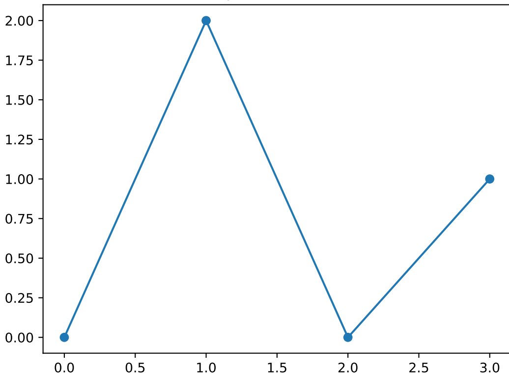
Shapelet number 25
