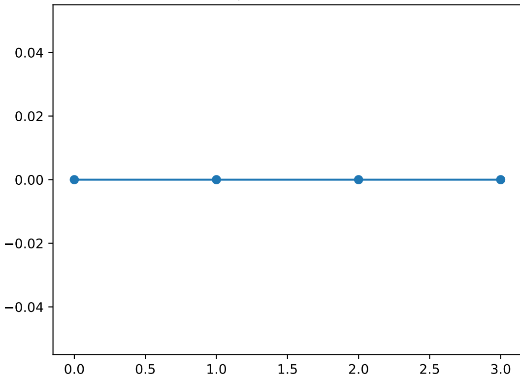
Shapelet number 20
