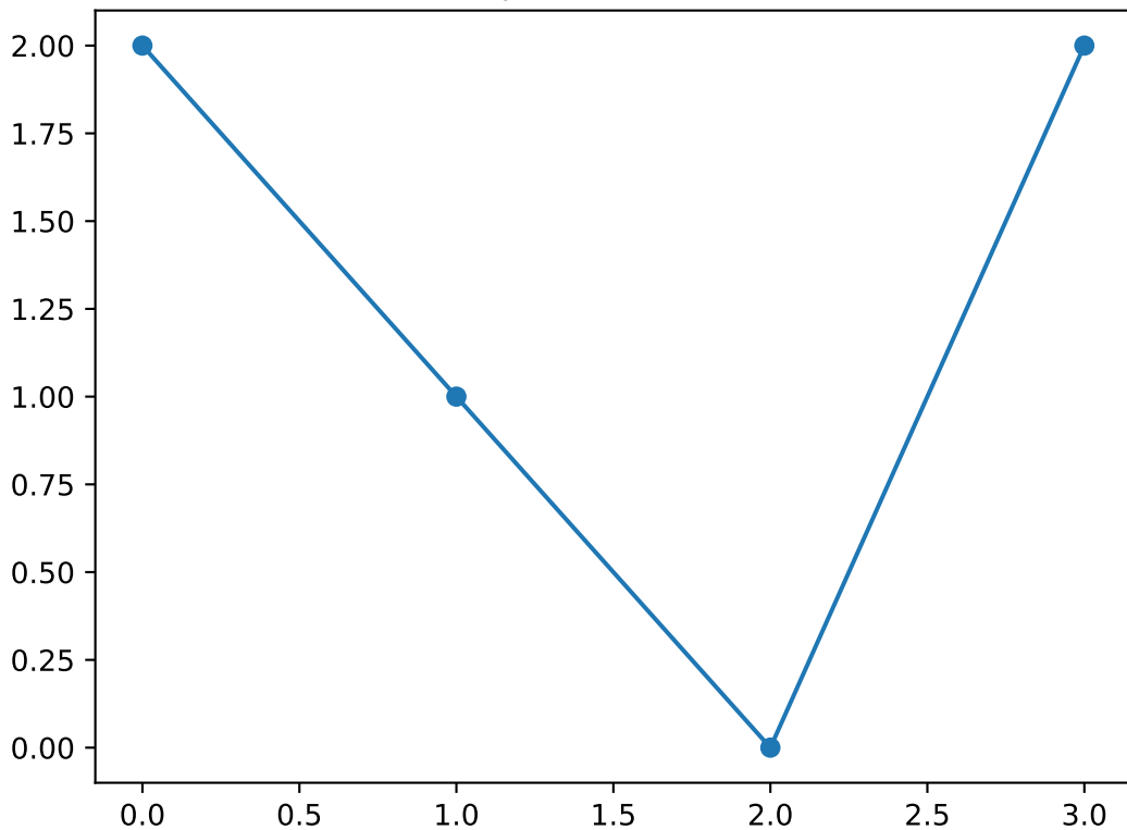
Shapelet number 56
