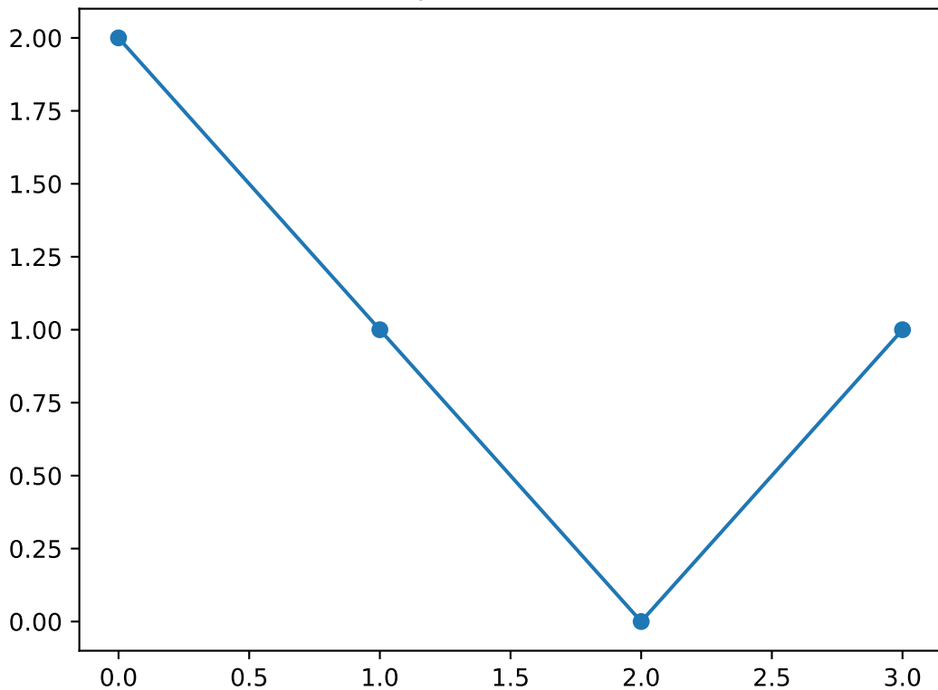
Shapelet number 55
