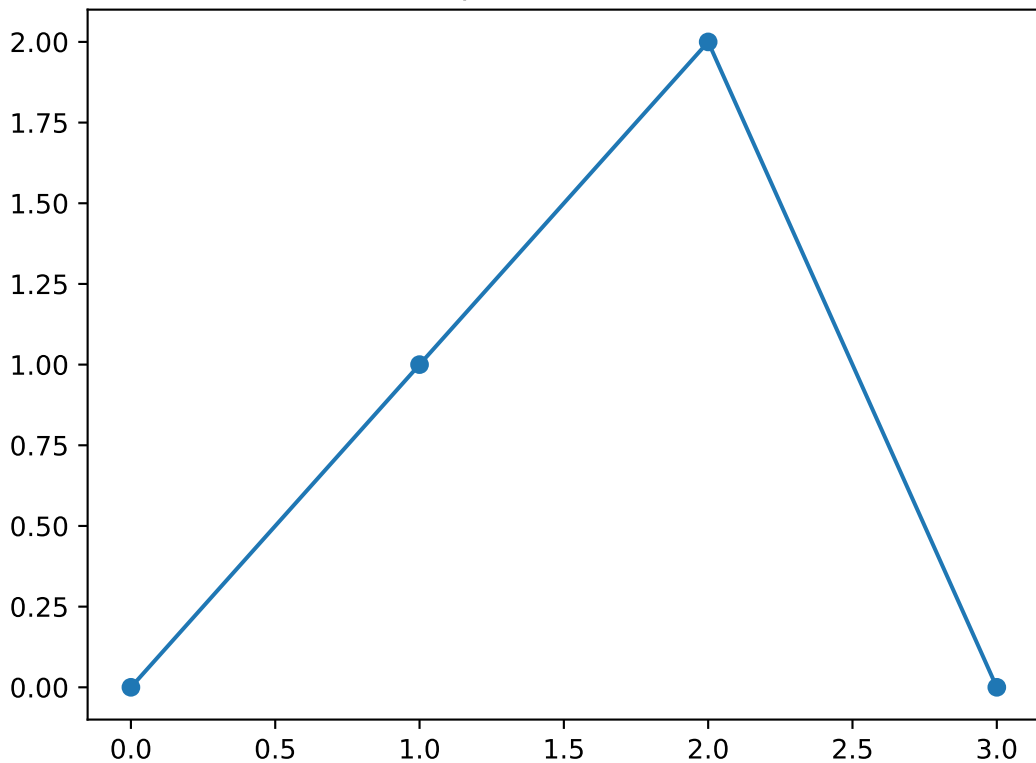
Shapelet number 22
