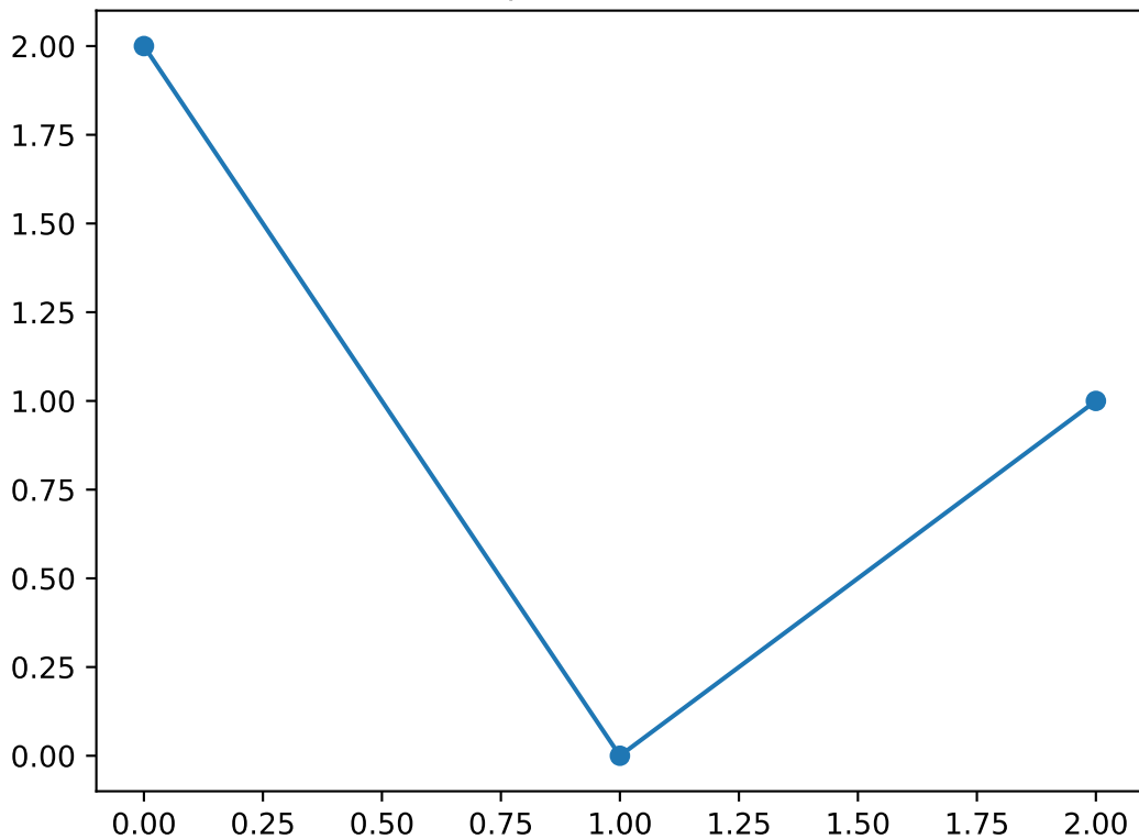
Shapelet number 12
