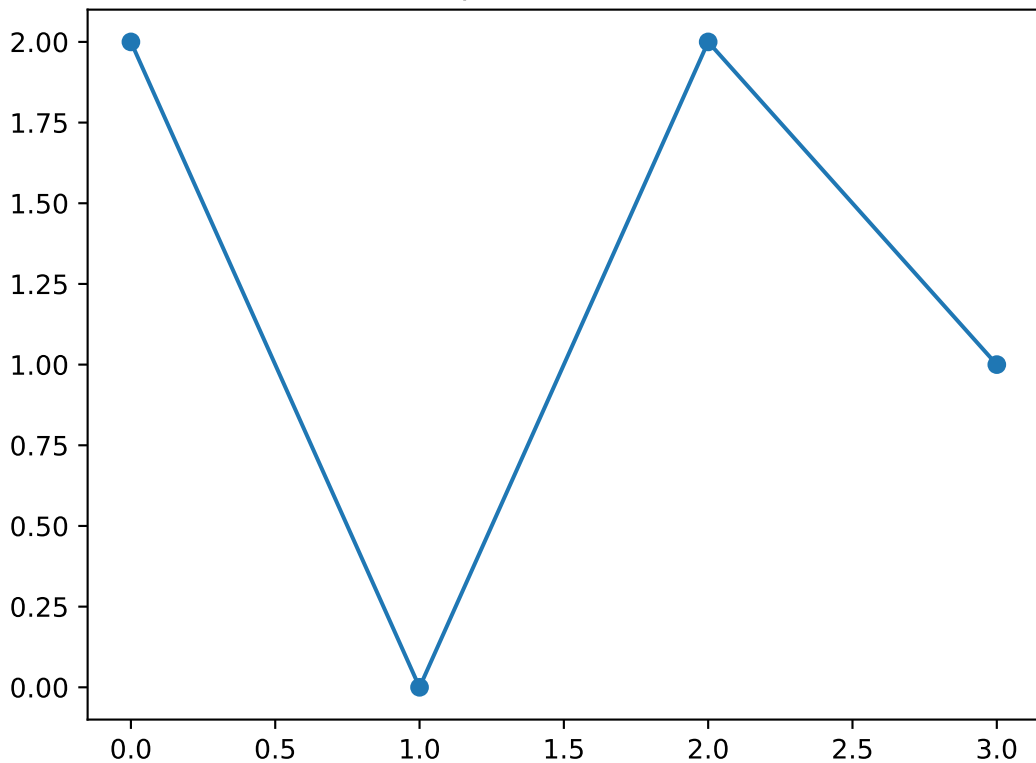
Shapelet number 52
