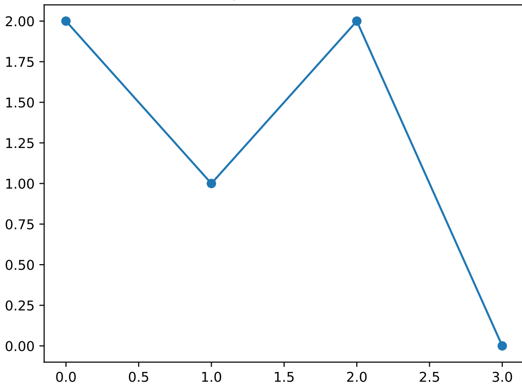
Shapelet number 65
