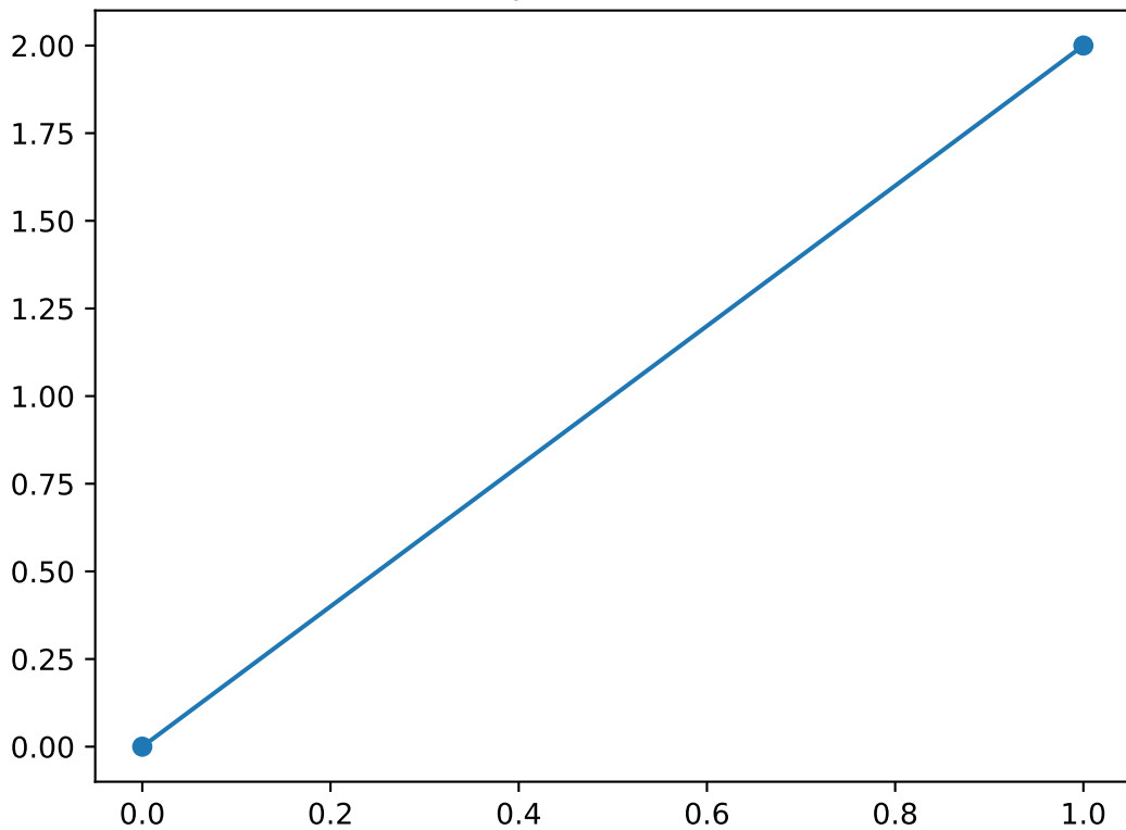
Shapelet number 1
