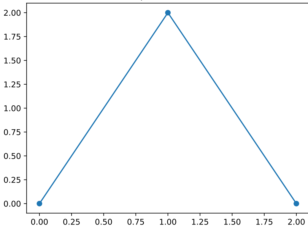
Shapelet number 6
