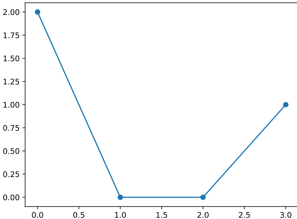
Shapelet number 46
