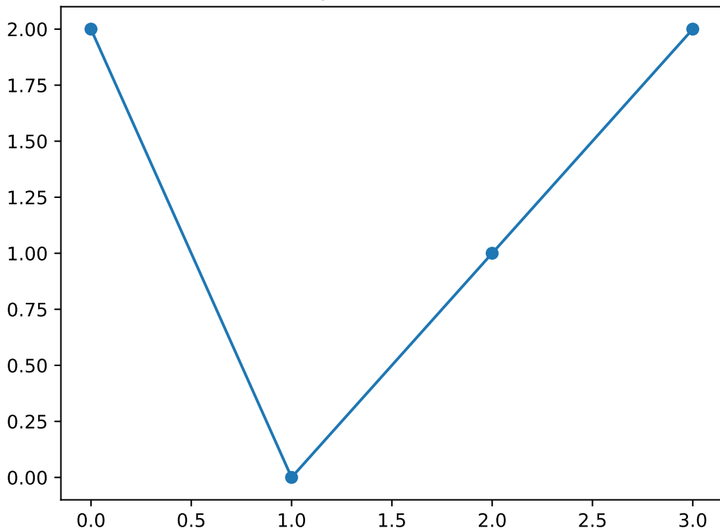
Shapelet number 50
