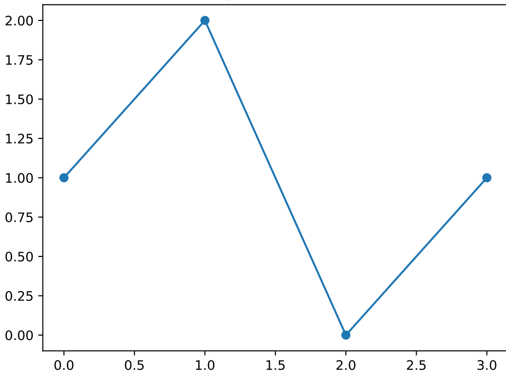
Shapelet number 41
