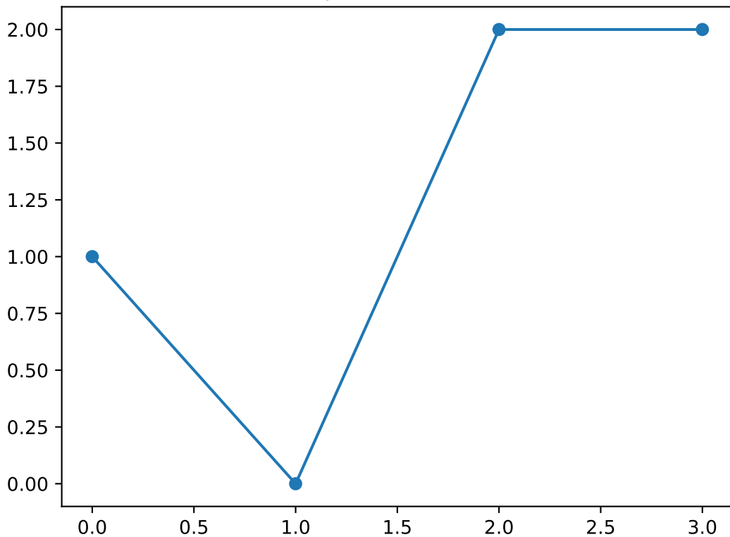
Shapelet number 37
