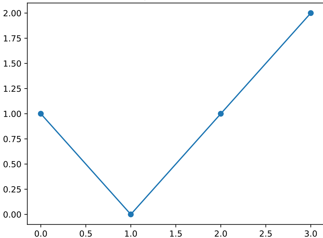
Shapelet number 34
