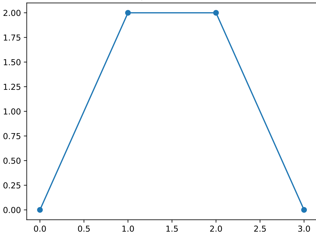
Shapelet number 30
