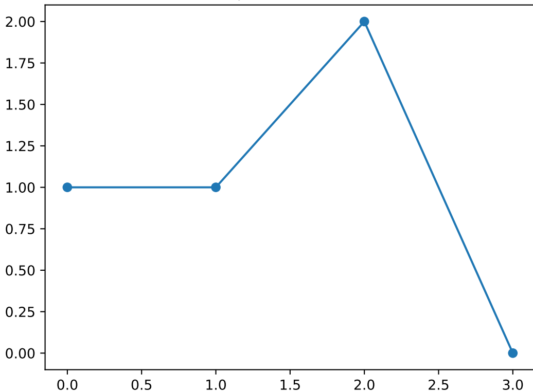
Shapelet number 39
