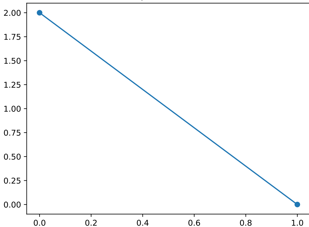
Shapelet number 2
