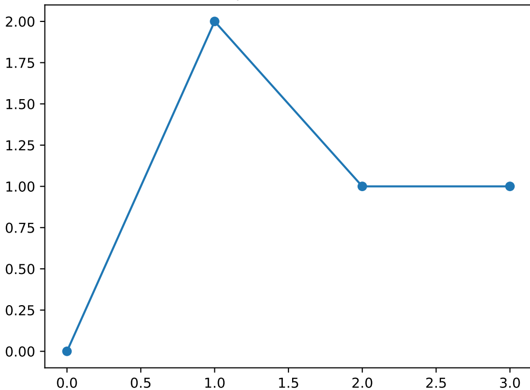
Shapelet number 28
