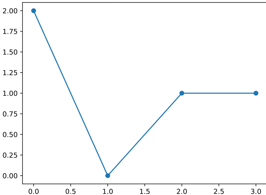
Shapelet number 49
