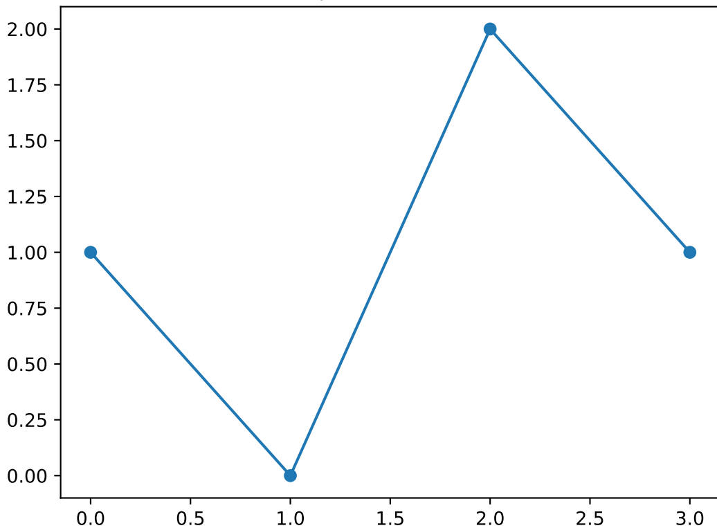
Shapelet number 36
