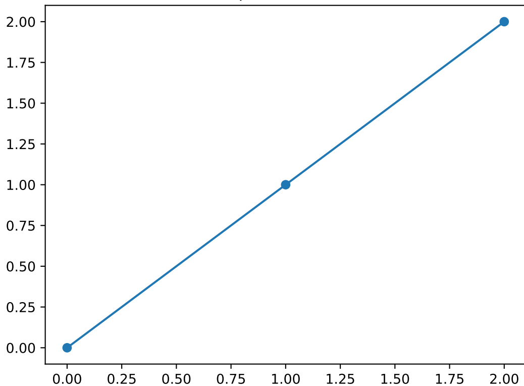
Shapelet number 3
