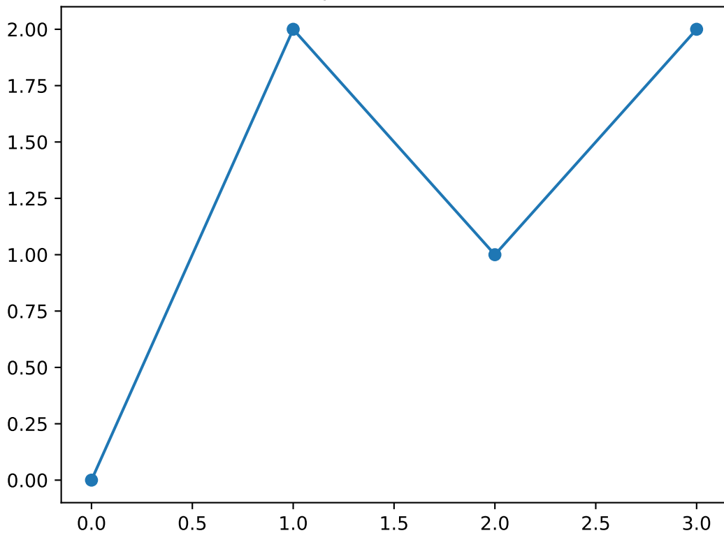
Shapelet number 29
