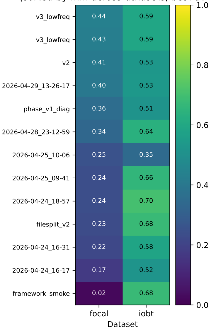
Cross-location type_f1 (sorted by min-across-datasets, best at top)
