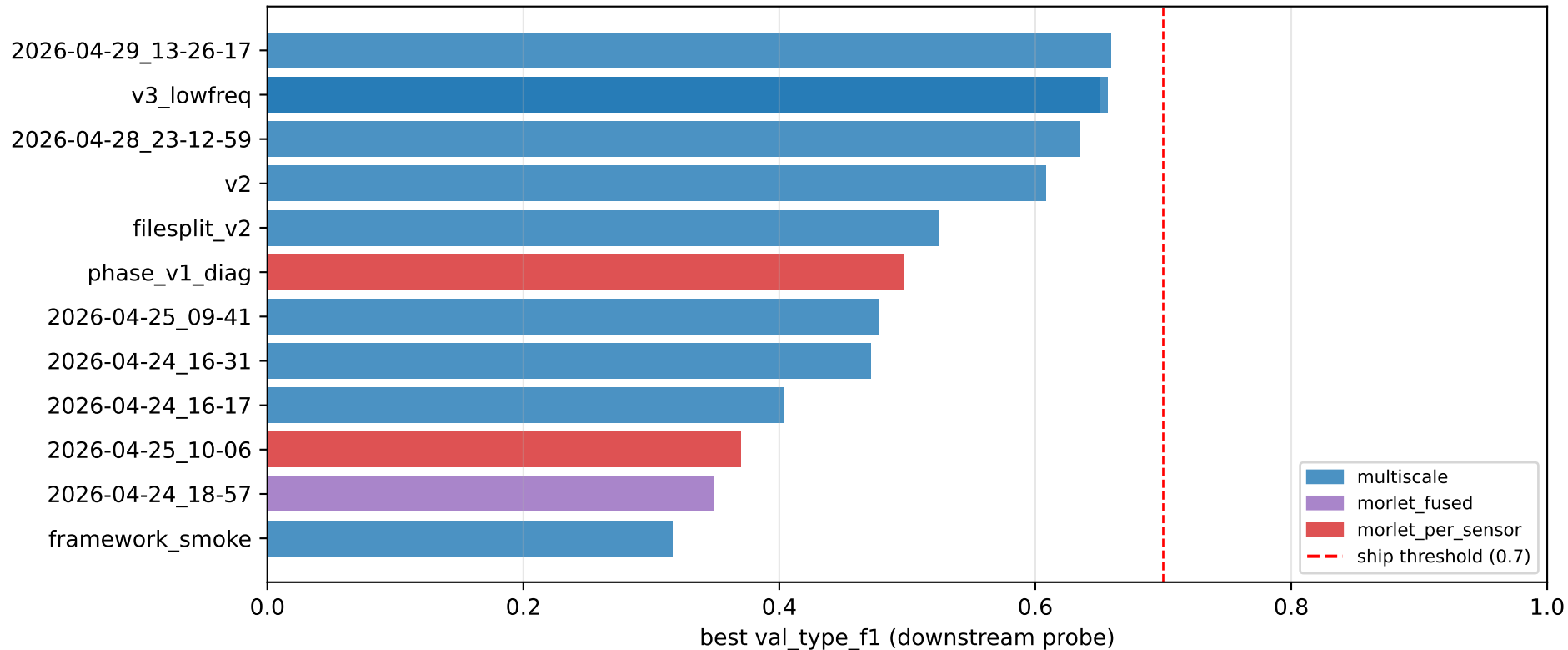
Best downstream type_f1 by run
