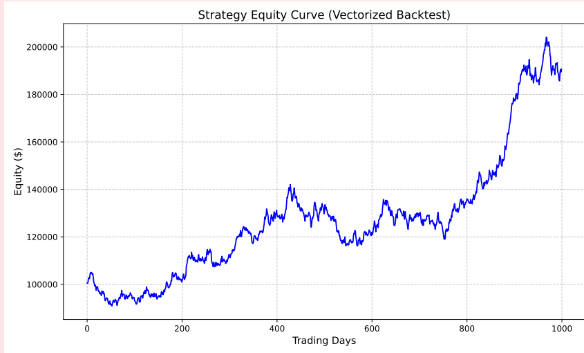
Figure 5.1: Equity Curve generated via pure NumPy vectorization.
