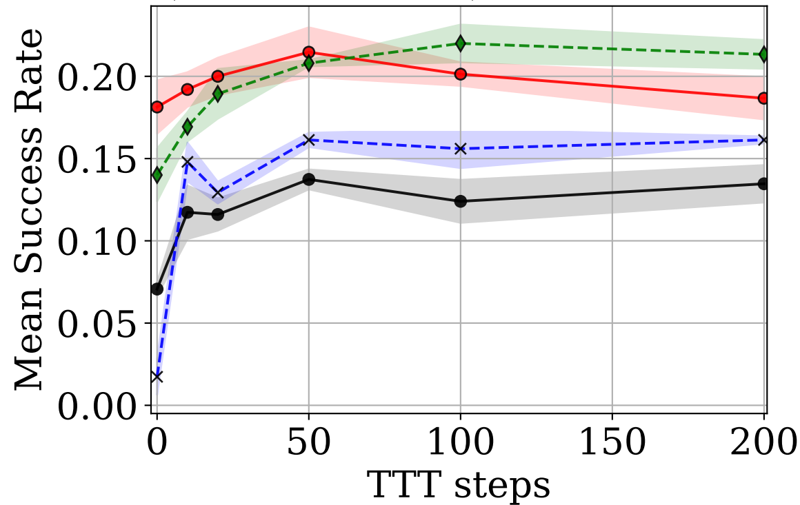
(Humanoidmaze) Critic-free BC
