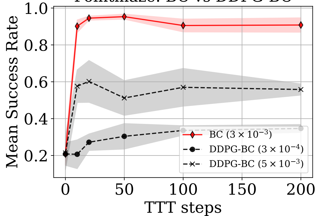
Pointmaze: BC vs DDPG-BC
