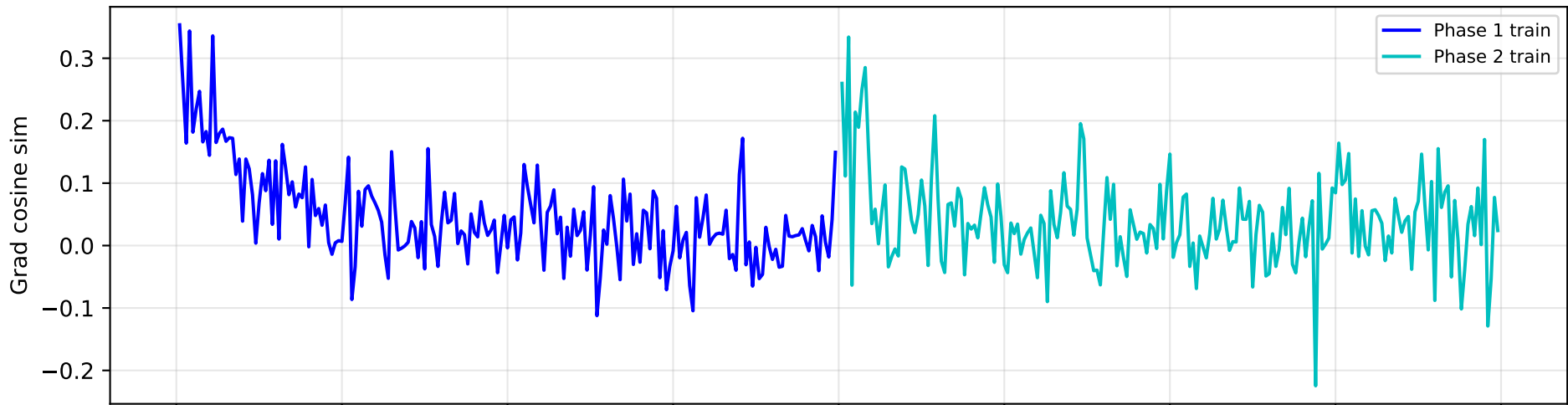
Gradient cosine similarity (current vs previous)
