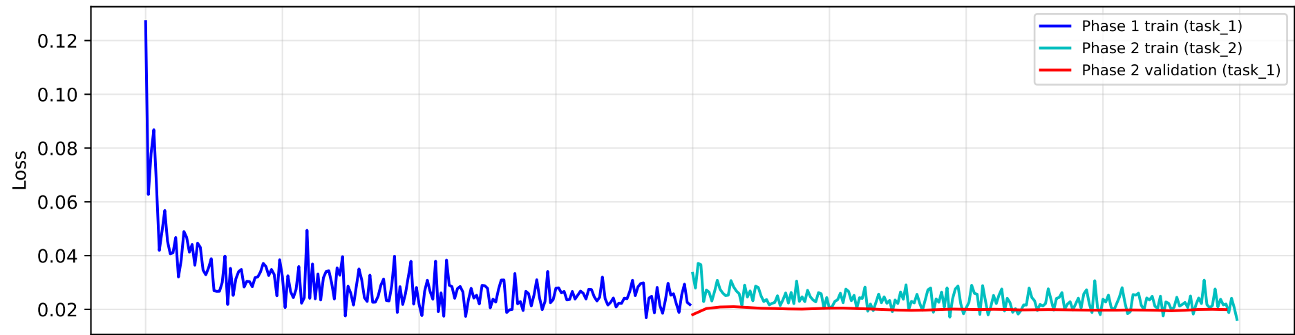
Fine-tune loss curves
