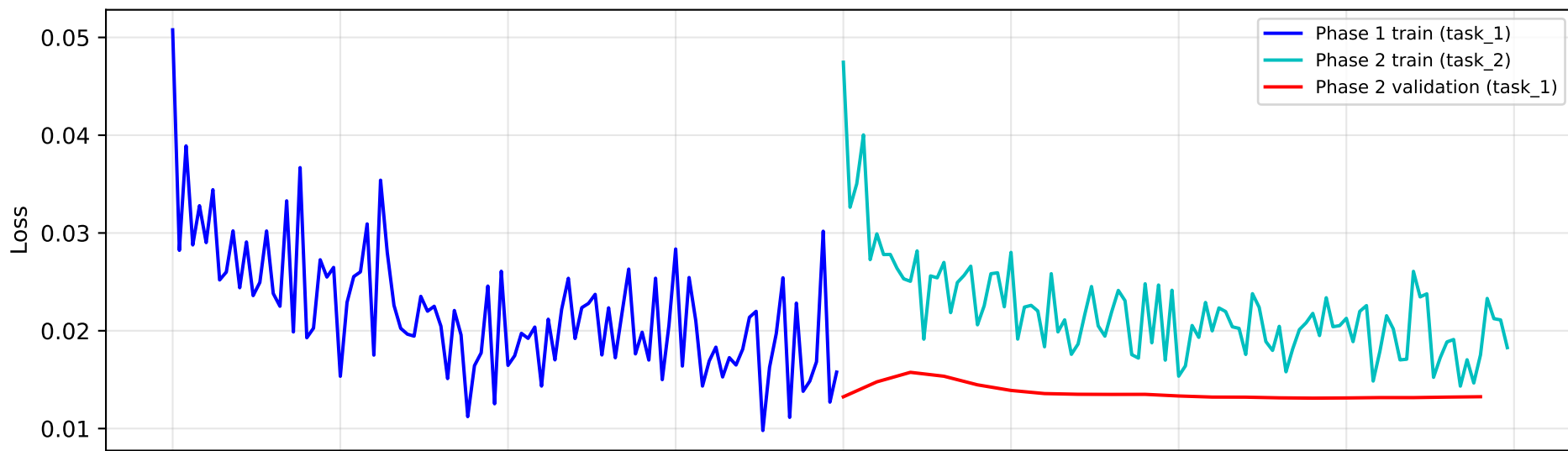
Fine-tune loss curves
