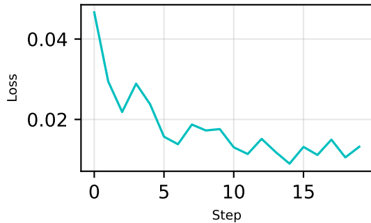
Student BC (outer iter 0)
